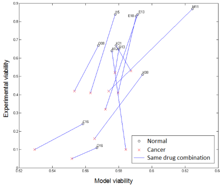
Figure 3. Computational versus experimental viability for IMR90 and A549. All drug codes shown are combined with A15 (a PDK1/AKT1/FLT3 Inhibitor). The experimental results are compared with the p=1 model predictions ( p=2 is similar). A positive slope means that there is positive correlation between the experimental and model results: the experiment showed that normal cells treated with (A15+O16), for example, fared better than cancer cells treated with the same drugs, which our model predicts as well. Note that while only 11 drug combinations are shown, 140 were tested, a promising 95% of which had a positive slope.
