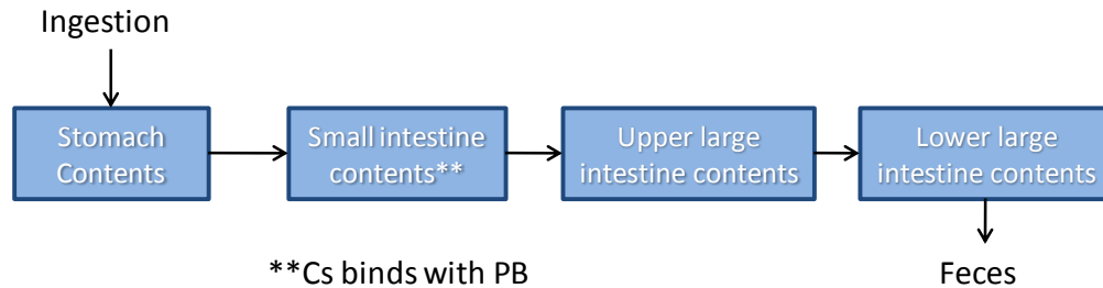
Figure 5. GI Tract Model for Prussian Blue Treatment
