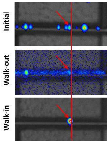
Fig. 7. Zoomed-in view of the EL images of the same device in Fig. 6. It is shown that the location that eventually becomes the dominant EL emission site after walk-in is also present in the initial and walk-out images.
