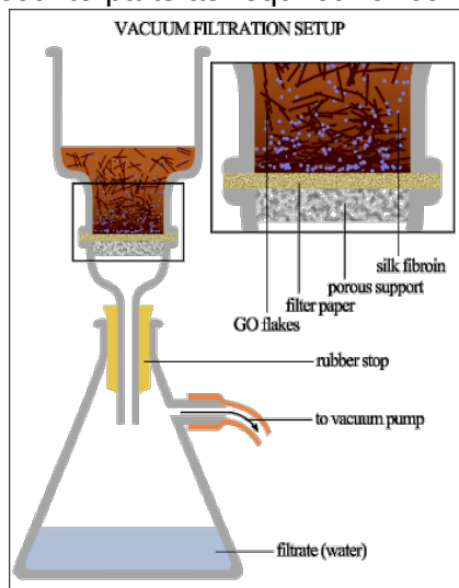
Experimental setup of the vacuum-assisted filtration system.
