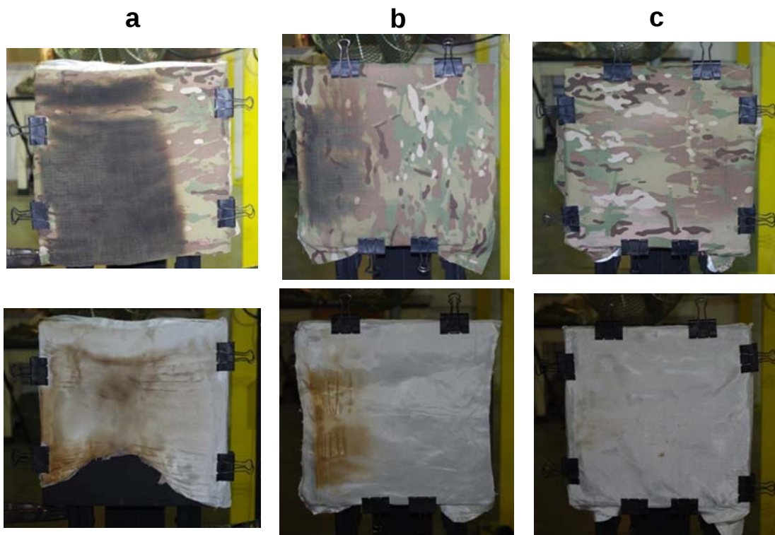
Figure A-1. Flat panel midscale test of Defender M and UHMWPE 375D with different clamping configurations: a) On two opposite sides only; b) On top and bottom only; c) On all four sides.
