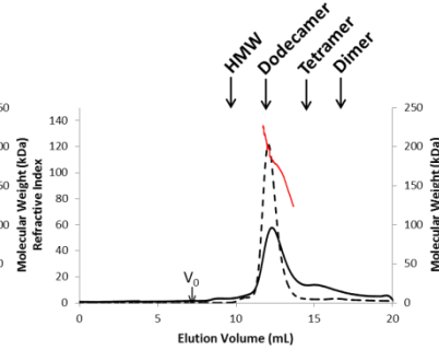
Figure A7.1: SEC/SLS data for tagged muteins: Analysis of tagged muteins generally showed a tendency toward the dodecameric state. This is in line with results for tagged wildtype and so gave no additional insight into the influence of the mutations. The exception was T104W which switched between the dimer and dodecamer even when the tag was attached (discussed in text). Tagged wildtype in identical conditions is shown with the dashed lines, molecular weight across the peaks with red lines.
