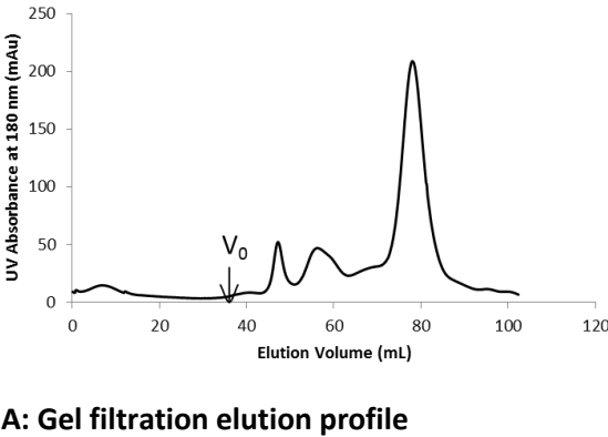
FigureA6.8: A: Typical gel filtration elution profile of the C47S mutein showed a single main peak around 80mL, with a number of early eluting peaks suggesting aggregation.
