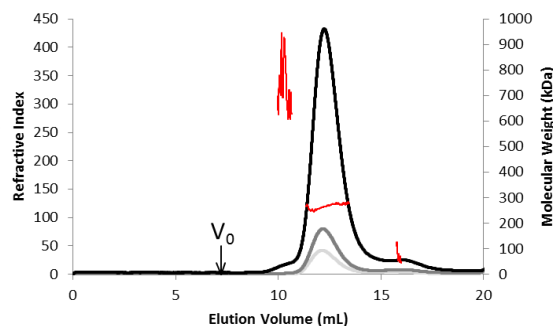
Figure 4.18: Oligomeric state of non-reduced HsPrx3 shows concentration dependence
