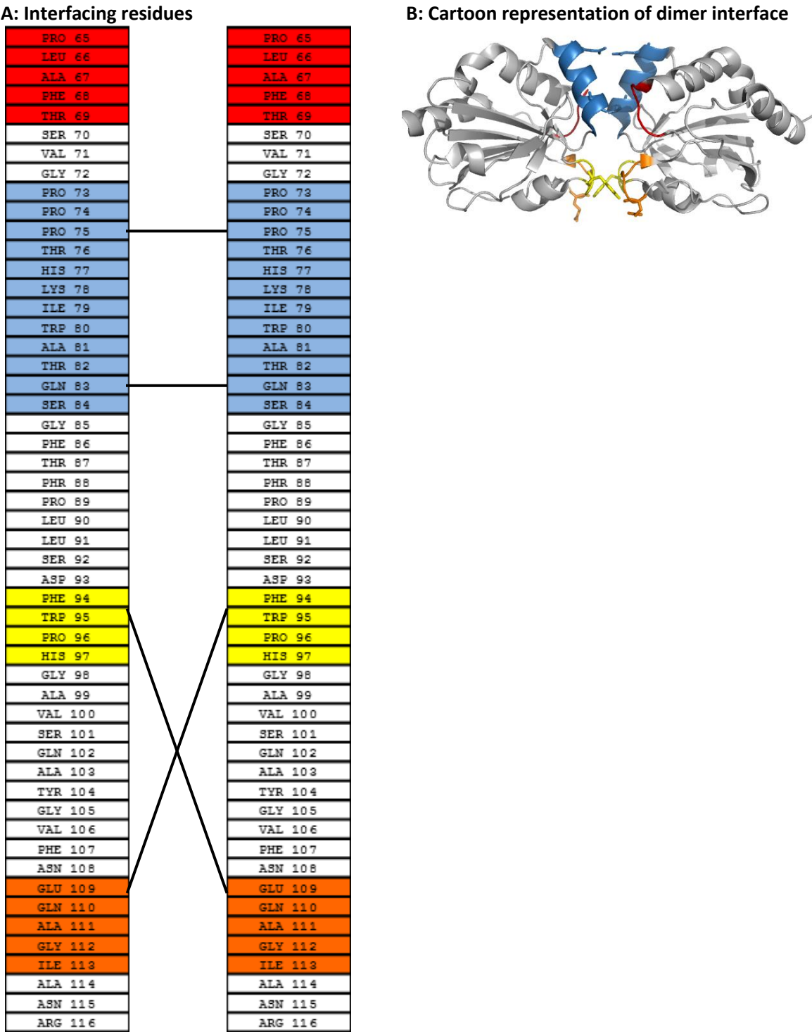
Figure 3.2: Interactions at the MtAhpE interfaces
