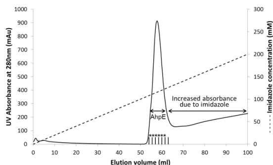
Figure 3.4: IMAC purification of wildtype MtAhpE
