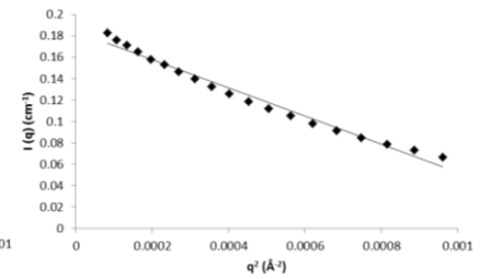
Figure A7.2: Guinier region plots of muteins: A number of muteins showed a nonlinear Guinier plot, indicative of aggregation. This was more common in non-reduced samples. R123G was particularly aggregated, as discussed in the text, and only one sample was able to be run through the in line FPLC. All other samples were injected directly into the capillary and analysed at 2 mg/mL (black diamonds); 1 mg/mL (dark grey diamonds); 0.5 mg/mL (light grey diamonds). Cleaved C47S was unable to be produced and the tagged construct was not able to be concentrated to higher than 1 mg/mL.
