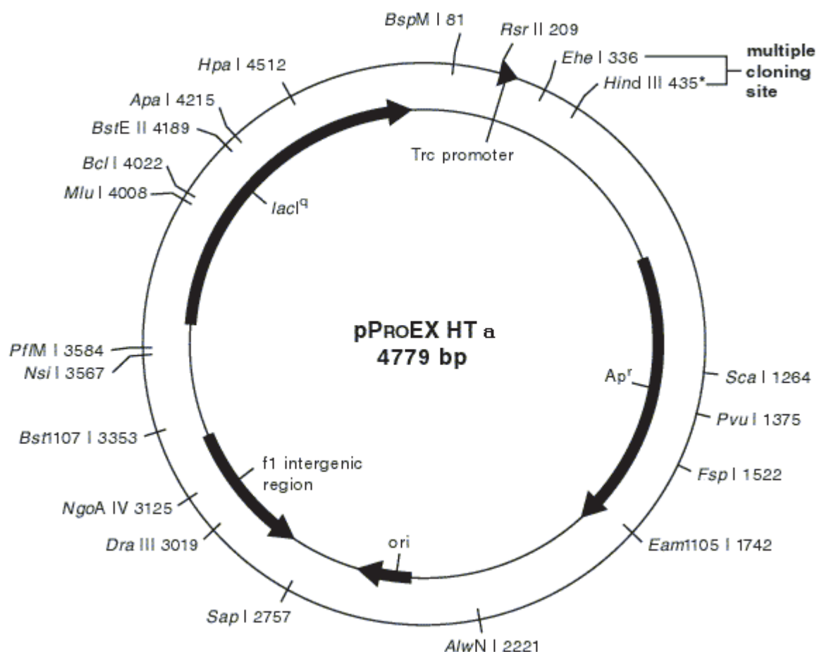
Figure A3.1: pProEX HTa vector map (Invitrogen): This vector was used for routine expression of MtAhpE protein.
