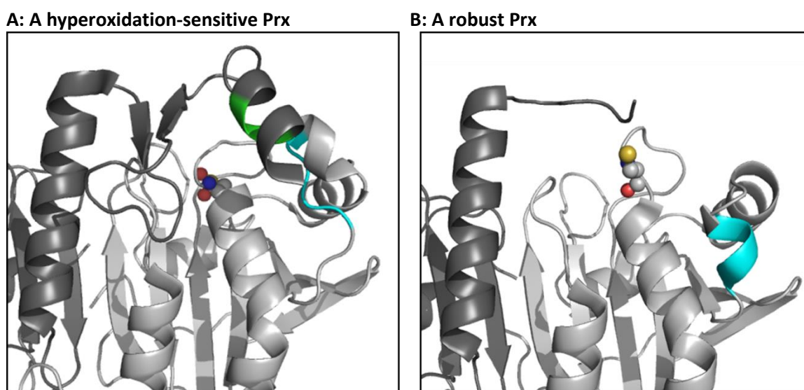
Figure 1.9: Prxs sensitive to hyperoxidation contain an additional helix
