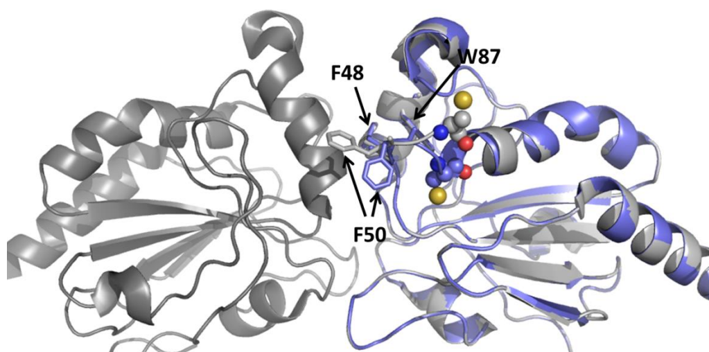
Figure 1.8: Individual residue movements contribute to interface dissociation
