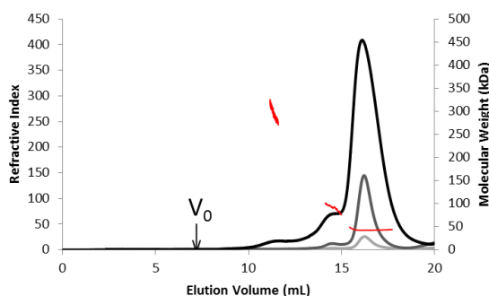
Figure 4.18: Oligomeric state of non-reduced HsPrx3 shows concentration dependence
