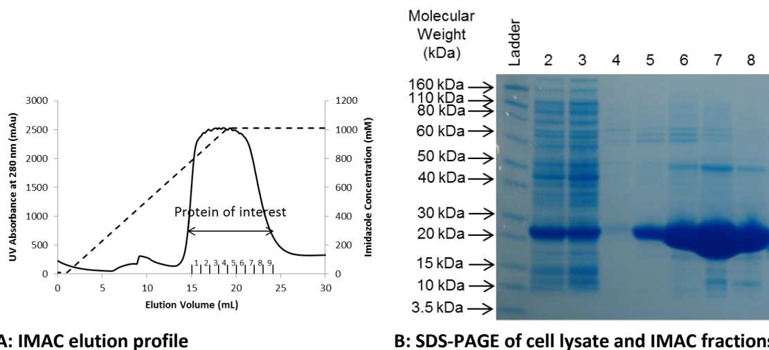
Figure A6.1: A: Typical IMAC elution profile of T104W mutein. B: SDS-PAGE gel showing: lane 2: whole cell lysate; lane 3: soluble fraction; lane 4: IMAC flow through; lane 5-8: selected fractions across the peak as indicated by stars on the chromatogram.
