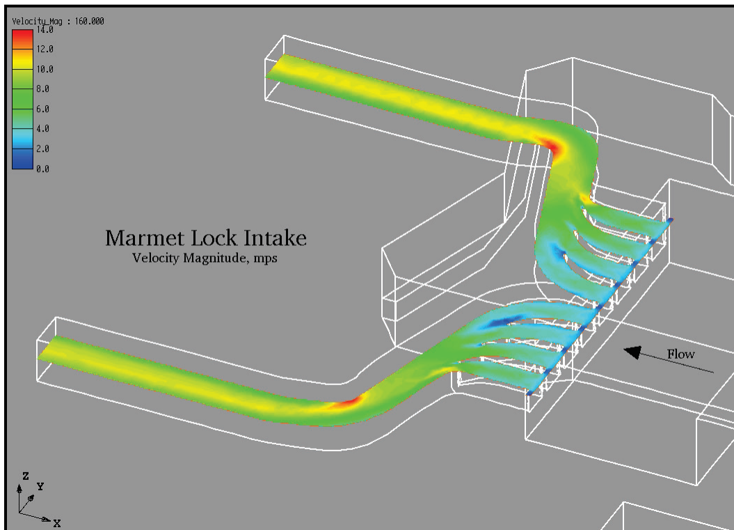
Figure 9. The 3-D computational flow model of Marmet Lock intake, velocity distribution along a plane through the culvert center (Stockstill and Berger 2000).
