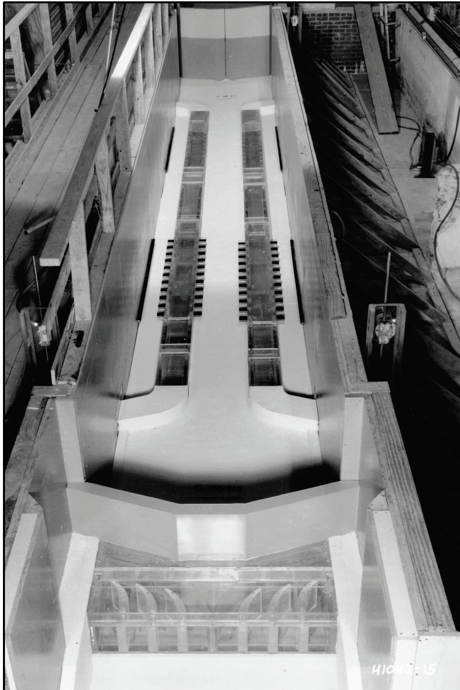
Figure 6. The 1:25-scale model of Marmet Lock filling and emptying system (Hite 1999).
