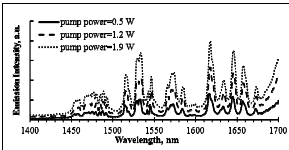
Figure 4. Spontaneous emission of 0.5% Er:YAG.
