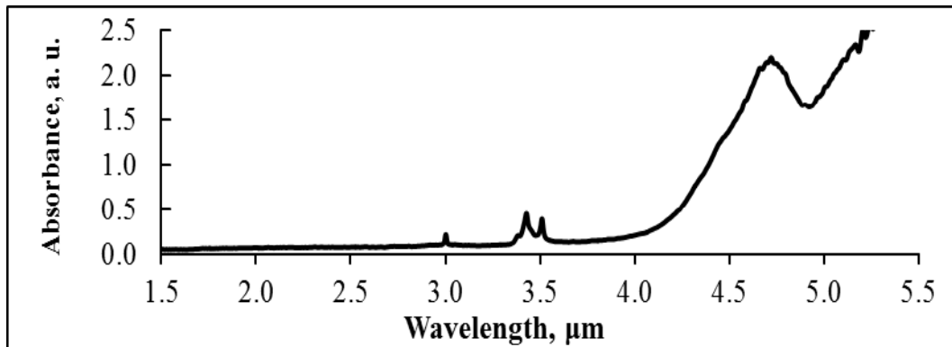
Figure 1. Absorbance of YAG. 3
