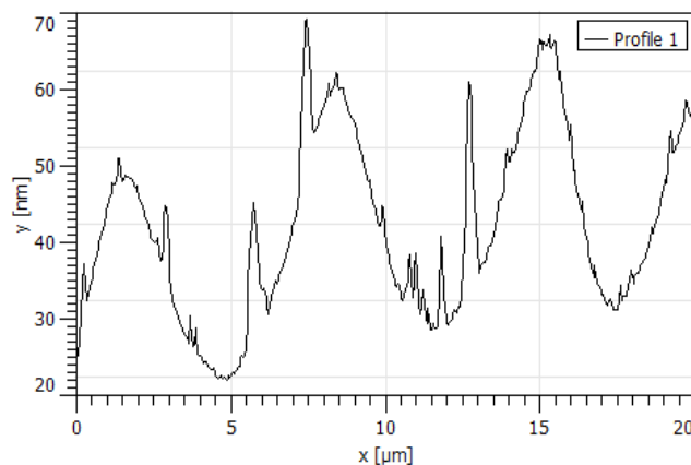
Figure 7. An AFM profile, showing the height of the facets.
