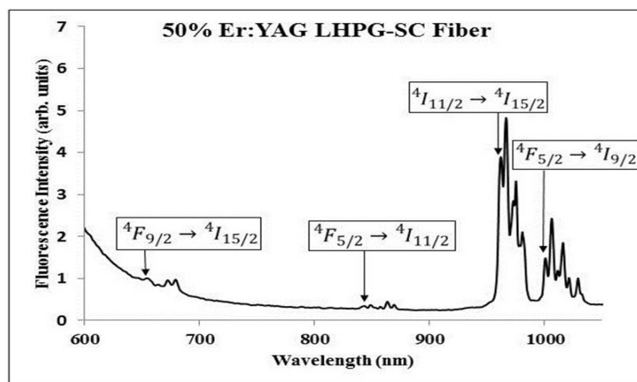
Figure 3. Energy transitions for erbium.
