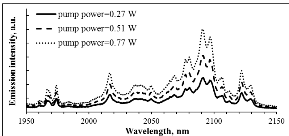
Figure 5. Spontaneous emission of 0.5% Ho:YAG.
