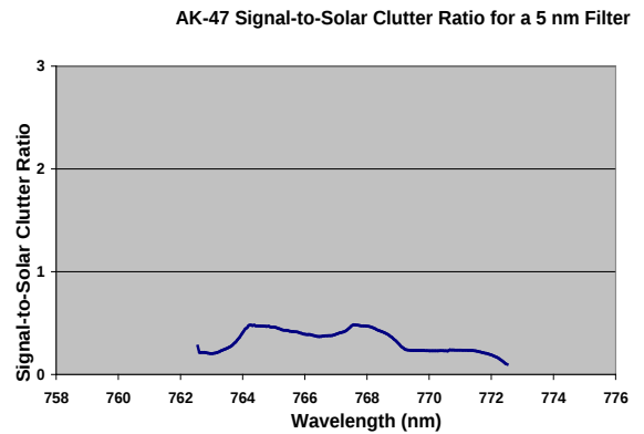
Figure 8. AK-47 muzzle Flash detected with a 5.0 nm FWHM filter.
