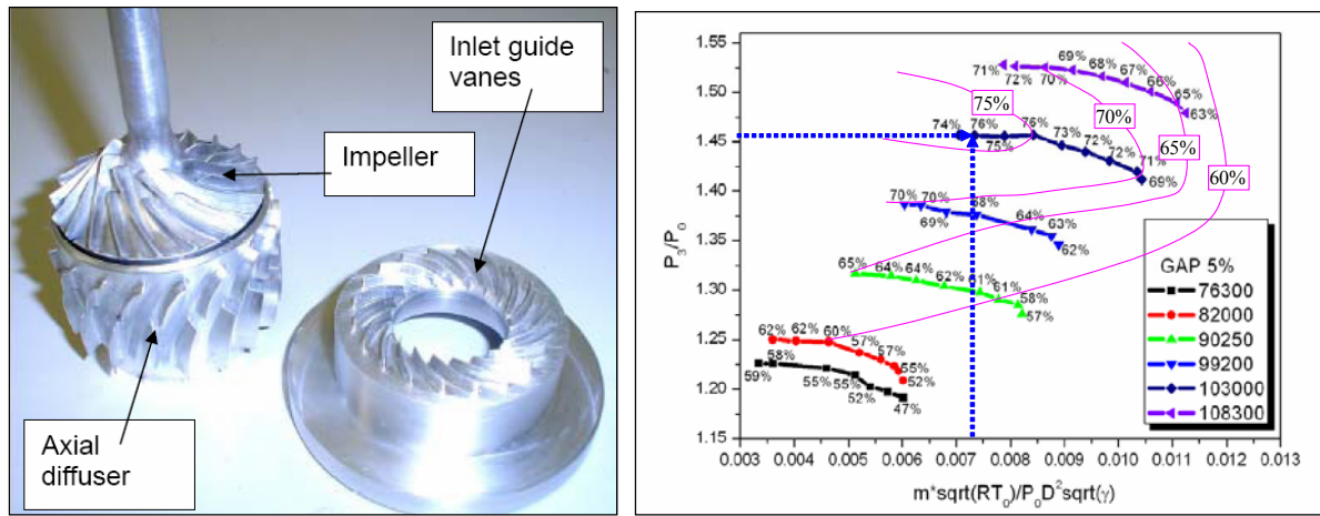
Figure 5: Photo & Performance plot of existing centrifugal compressor
