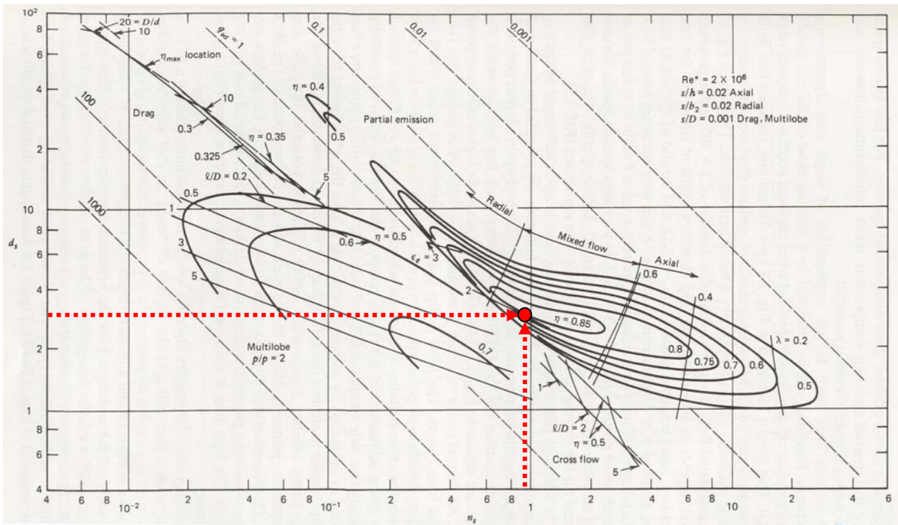
Figure 4: n_s d_s diagram for single stage compressors [1] .
