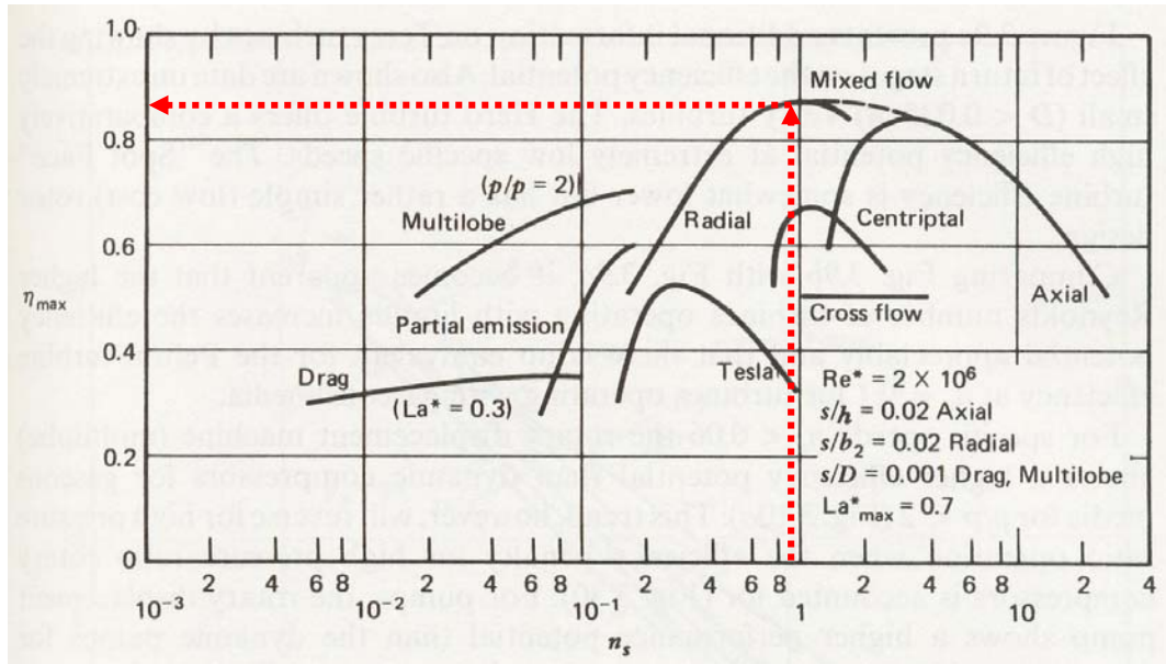
Figure 3: Maximum compressor efficiencies as a function of specific speed (various types) [1] .
