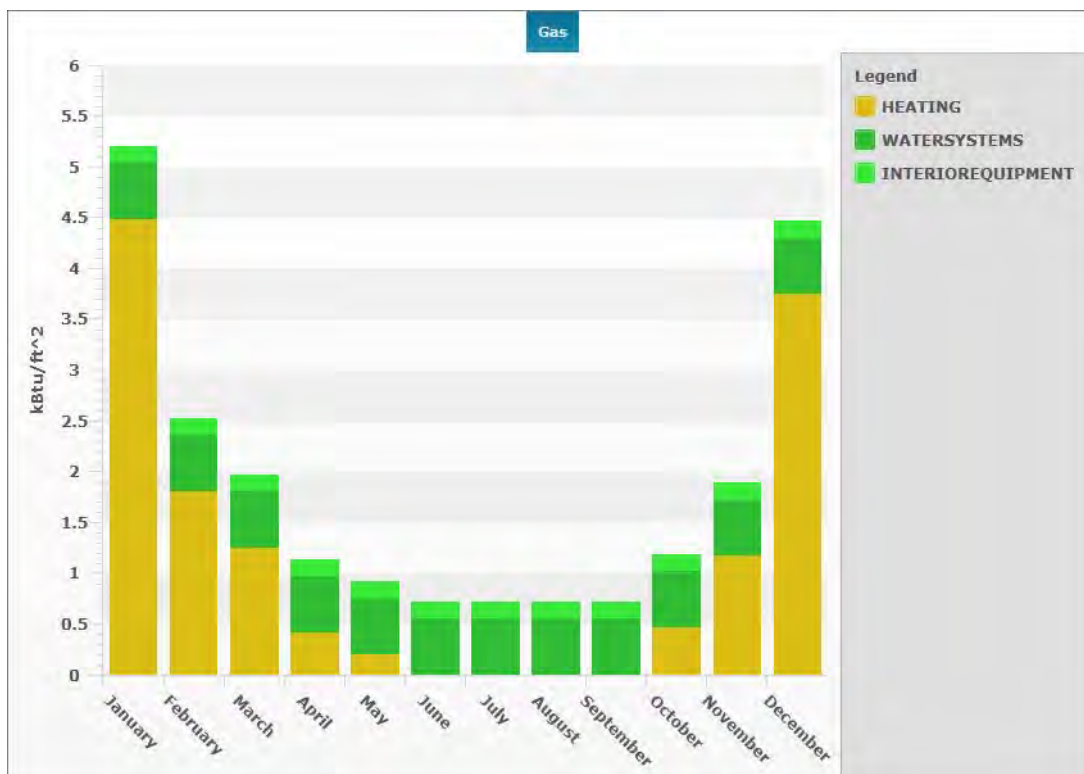
Figure 14. Natural gas consumption by end use.
