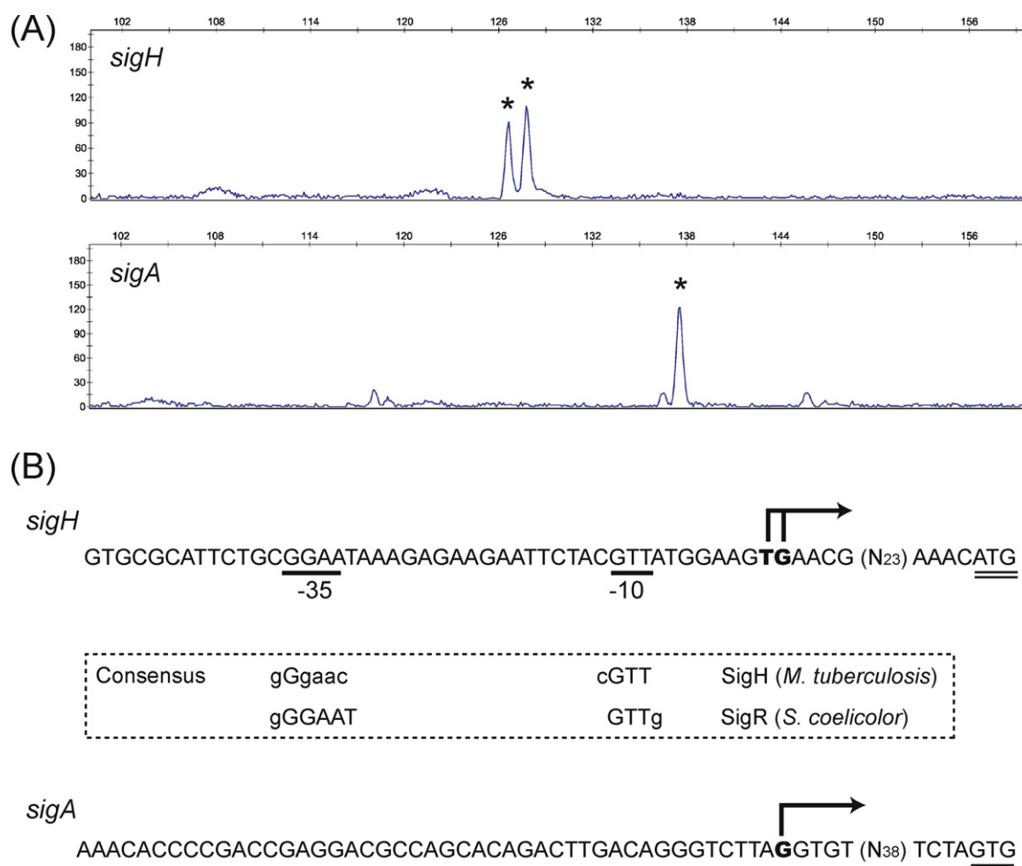
Fig. 4 – Putative SigH binding and transcription starting sites in upstream of sigH . (A) Primer extension electrophoregrams of the upstream regions of sigH and sigA . (B) The sequences of the sigH and sigA upstream regions are shown, and transcription initiation sites are indicated with bent arrows. Lines under the sequences correspond to the putative SigH-dependent promoters. Double lines under the sequences correspond to the start codon of sigH or sigA genes. The consensus sequences recognized by SigH of M. tuberculosis and SigR of S. coelicolor are shown at the bottom. Nucleotides of the consensus sequence conserved in more than 80% of the sequences are in capital letters.
