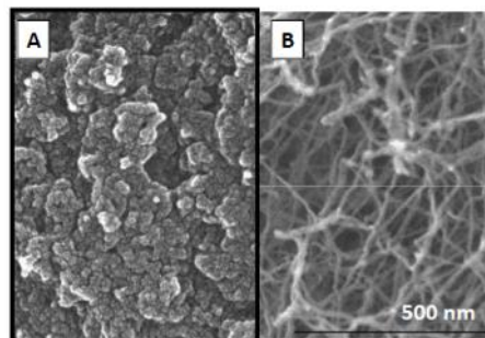
Fig. 8. (A) PI-AMN ( \rho_b=0.186 \text{ g cm}^{-3} , II=87\% \text{ v/v} , \rho_s=1.453 \text{ g cm}^{-3} , BET surface area= 431 \text{ m}^2 \text{ g}^{-1} ). (B) PI-ISO ( \rho_b=0.090 \text{ g cm}^{-3} , II=94\% \text{ v/v} , \rho_s=1.473 \text{ g cm}^{-3} , BET surface area= 315 \text{ m}^2 \text{ g}^{-1} ) [11a,11b].
