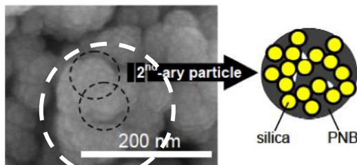
Fig 2. Polynorbornene (PNB)-crosslinked silica aerogels via ROMP. Yellow-filled circles: Primary particles. Black dashed circles: secondary particles. White dashed circle: network-forming aggregates. (The greatly improved mechanical properties are attributed to polymers confined within secondary particles, hence invisible by SEM [20].)
