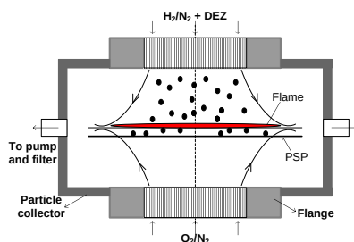
Fig. 1 Schematic showing of the CDF reactor for making metal oxide nanoparticles.
