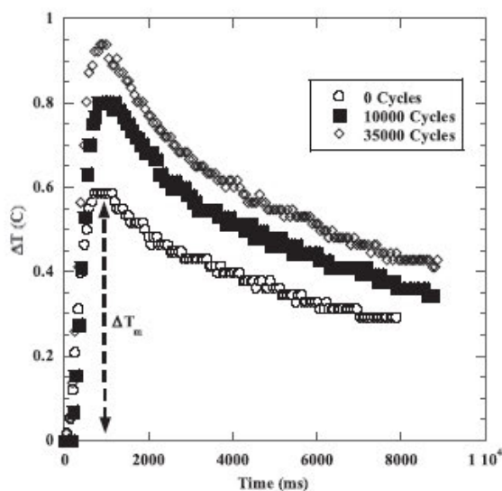
FIG. 2. Time-temperature curves in as received and fatigue damaged Ti-6Al-4V sample.
