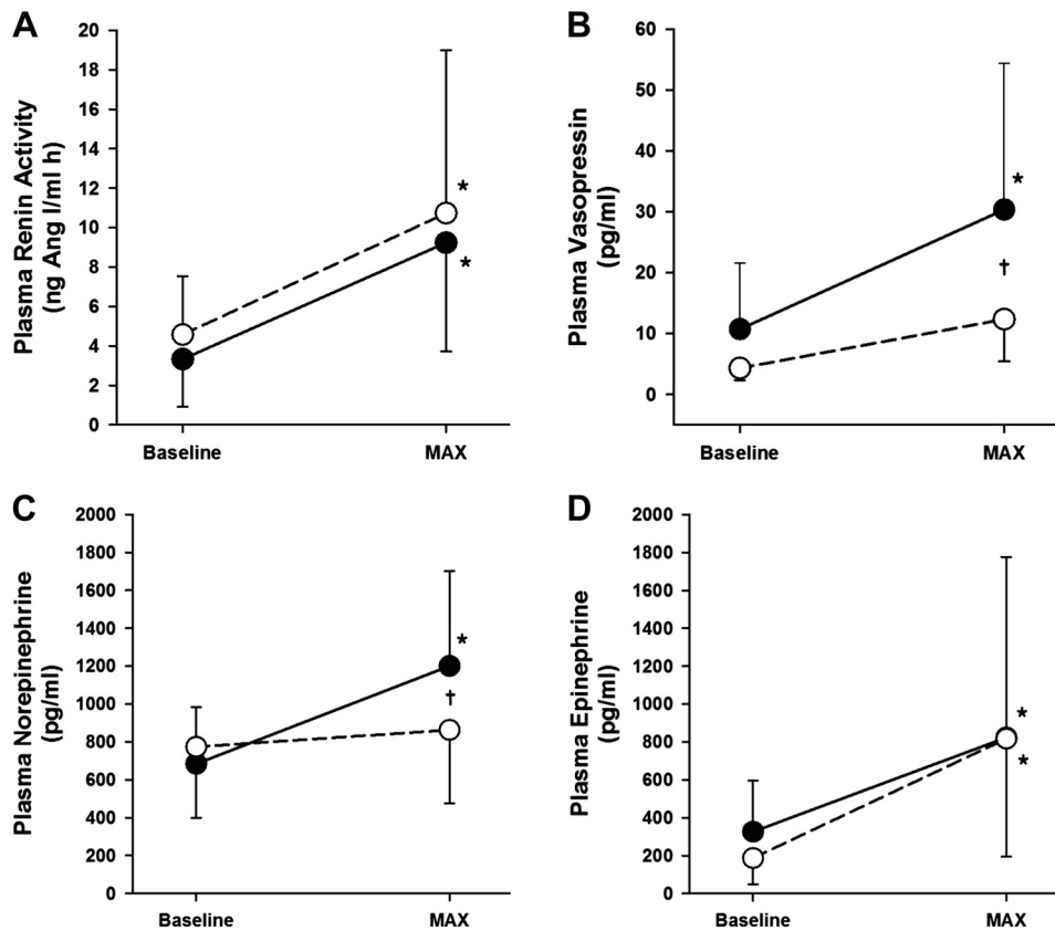
Fig. 5. Plasma renin activity (A), vasopressin (B), norepinephrine (C), and epinephrine (D) are shown at baseline of hemorrhage (●, solid lines) and matching LBNP (○, dashed lines), and at the maximum level of hemorrhage and matching LBNP (MAX). Values are means \pm SD; n = 12 . *Difference from baseline ( P < 0.01 ). †Difference between hemorrhage and LBNP ( P < 0.01 ).
