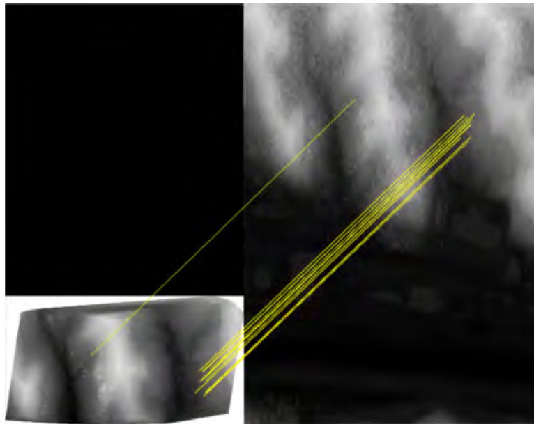
Figure A.56: This swatch matched 12 features in forest for an 3D aircraft position magnitude error of 5.05 meters. Close inspection shows 2 matches are weak outliers.
