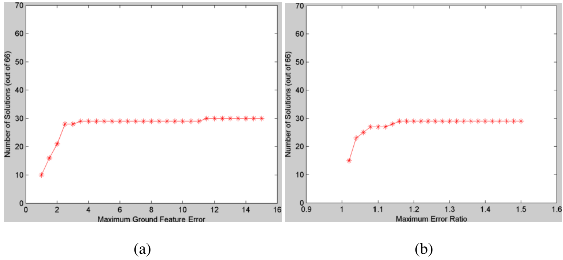
Figure 4.5: The number of swaths that resulted in a position estimation in relation to changes in (a) threshold parameter \alpha and (b) threshold parameter \beta , while the other thresholds are held constant.
