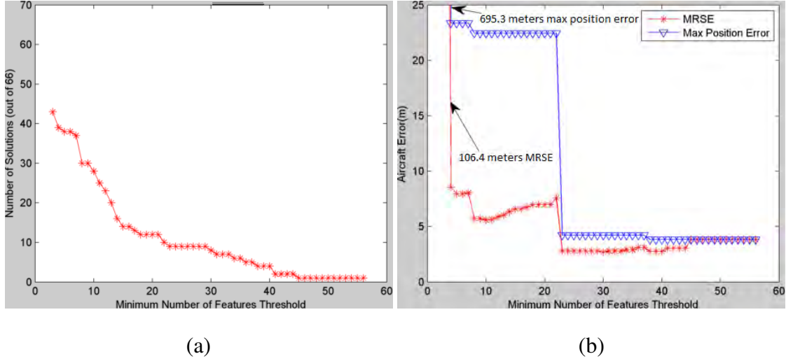
Figure 4.9: Example where threshold \alpha is held at 50 meters and threshold \beta is held at 2, while threshold \gamma is allowed to vary against (a) the number of swaths that resulted in a position estimation and (b) the MRSE of all the position estimates in the flyover, with the flyover largest position error magnitude.
