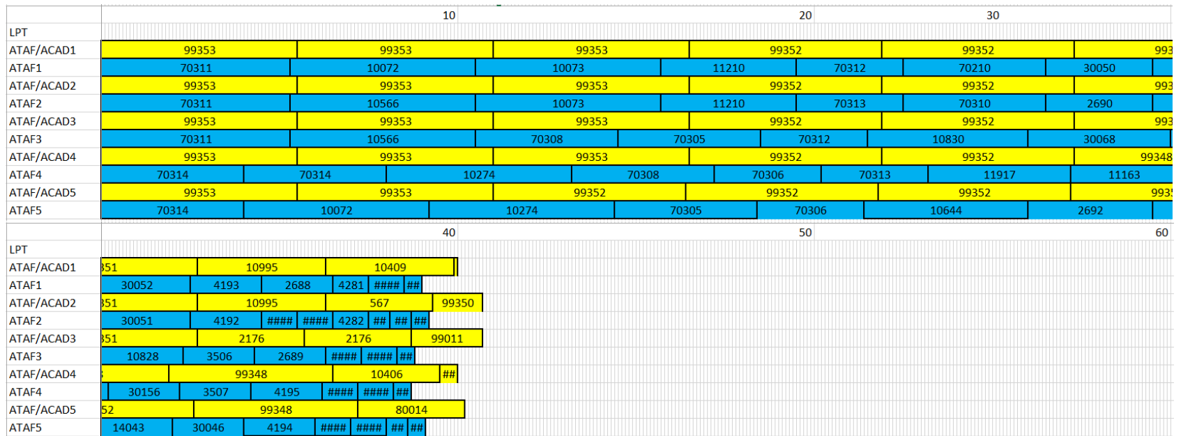
Figure 3: Scheduling, LPT
