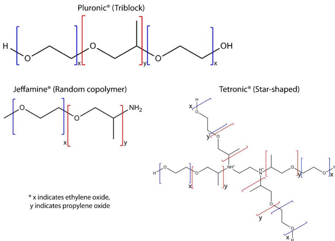
Figure 2. Chemical architectures of polymers comprising ethylene oxide and propylene oxide groups.
