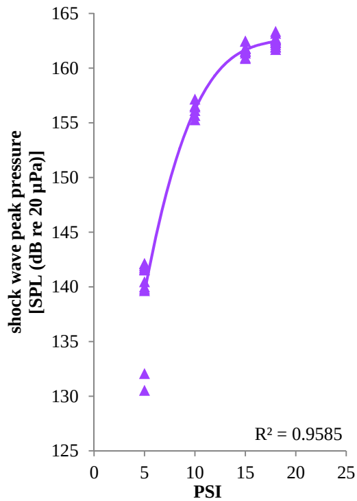
Figure 10. 1-mil (a), one sheet, third-order polynomial fit.
