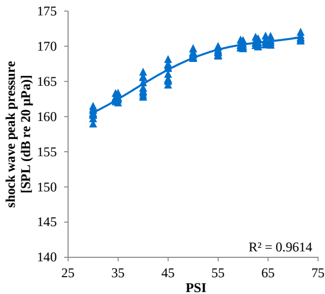
Figure 6. 2-mils (a), one sheet, third-order polynomial fit.
