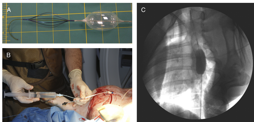
Figure 1. A, Single component PBS designed to be positioned and inflated without fluoroscopy. The lead or insertion end is a floppy tipped 0.035-inch wire fused to the compliant balloon catheter. A collapsible nitenol rail system is positioned between the floppy tip of the wire and the compliant balloon for the purpose of centering the system within the axial arterial lumen as the device is inserted and positioned. B, Photograph of the PBS having been inserted through an 8 Fr right femoral artery sheath. The syringe is filled with a mixture of contrast agent and saline for balloon inflation. C, Fluoroscopic image of the PBS inflated in the thoracic aorta with the floppy wire tip and flexible nitenol rail system proximal to the inflated balloon.
