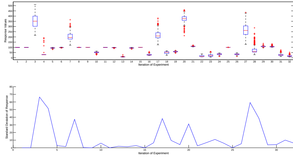
Figure 13. Boxplot and Standard Deviation of Response
