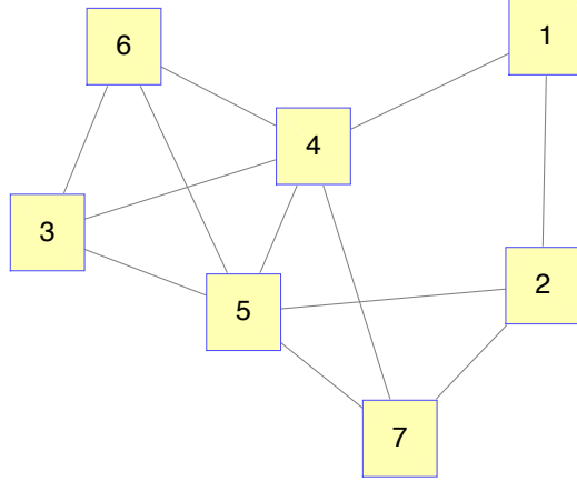
Figure 6. Network on 7 nodes and 12 edges
