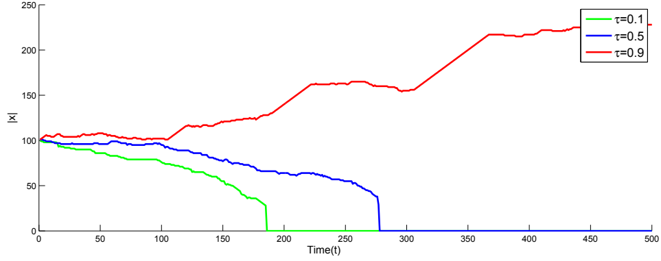
Figure 33. \tau and Size of the Largest Component |x_t|
