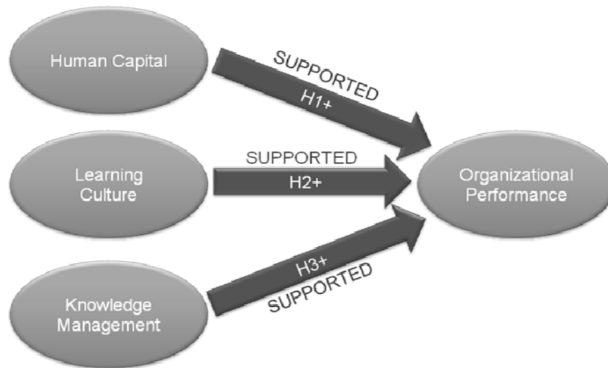
Figure 11: Theoretical Model
