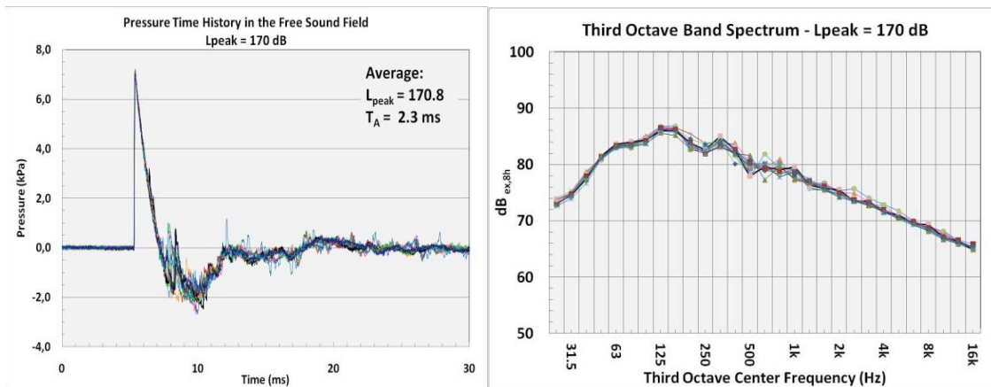
Figure 12: Pressure time history and 1/3 octave band spectrum for the 170 dB SPL noise level
