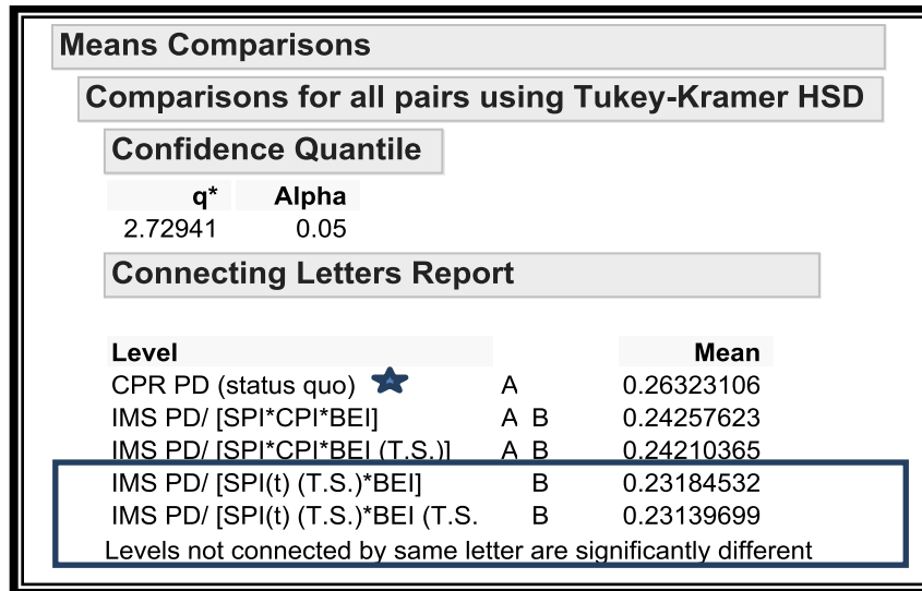
Figure 25: Tukey-Kramer HSD (OTB)
