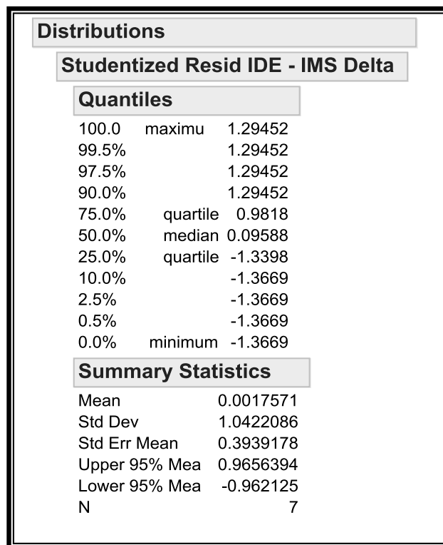
Figure 97: Studentized Residuals Check for Outliers (IDE - IMS Delta)
