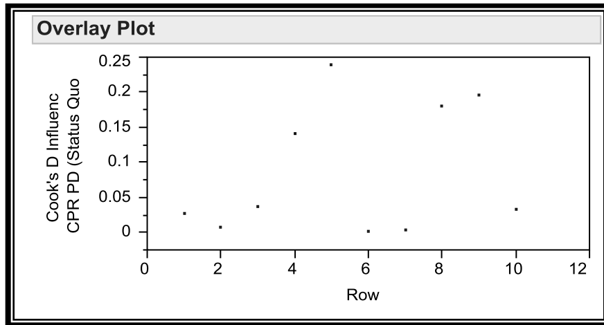
Figure 56: Cook's D - CPR PD (status quo)
