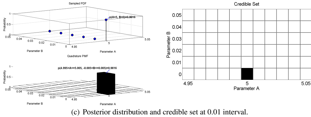
Figure 3.12: Left: PMFs for the multiple parameter estimate of An + B . Parameters used are A = 5 , B = 0 and N = 5000 . Right: Resulting 90% credible regions. Note: interval size decreases from top to bottom.
