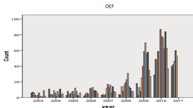
Figure 4. Month-by-month number of facial and penetrating neck injuries in Operation Enduring Freedom.
