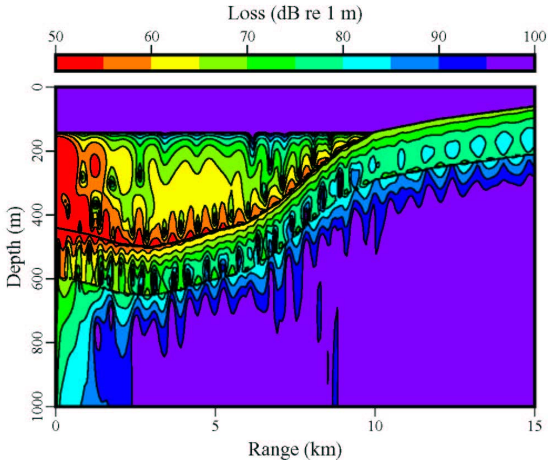
Figure 1. Many propagation problems involving range-dependent transitions between water and elastic sediments can be handled efficiently and accurately using a hybrid PE approach. Transmission loss contours, to 1000 m in depth and 15 km in range for a 5 Hz source, are shown for a model beach environment. The ocean depth is 300 m at the initial range (where the source is 5 m above the bottom), then increases to a maximum of 360 m at about 3 km, and finally decreases with variable slope to zero at 10 km. An elastic sediment layer is 150 m thick and follows the bathymetry for the first 10 km, after which its upper surface forms a beach that rises with uniform slope to 80 m above sea level at 15 km. The sediment layer has compressional and shear sound speeds of 2400 and 1200 m/s, corresponding attenuations of 0.05 and 0.1 dB/ \lambda , and density 1.5 gm/cm 3 . The basement below the elastic layer has higher sound speeds and density. The contours illustrate a conversion between interfacial wave types. A Scholte wave develops at the water-sediment bathymetry, and the energy in this wave moves into a Rayleigh wave at the air-sediment boundary.
