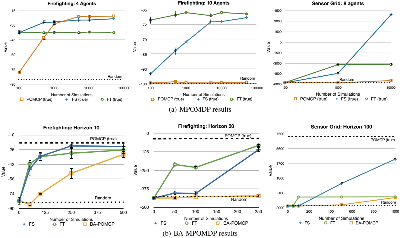
Figure 4: Results for (a) the planning (MPOMDP) case (log scale x-axis) and (b) the learning (BA-MPOMDP) case for the firefighting and sensor grid problems.
