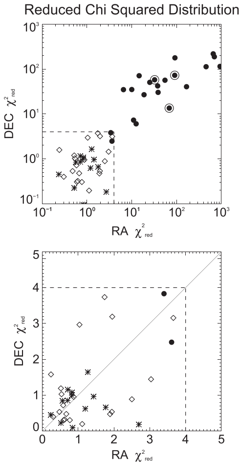
Figure 3. Reduced chi-squared ( \chi^2_{\text{red}} ) values comparing the astrometric residuals to the case of perfectly flat residuals, i.e., an exact astrometric solution with no perturbation. The lower panel is a zoom of the dotted square region in the upper. Asterisks represent the 13 stars without close stellar secondaries analyzed in this paper. Diamonds represent additional calibration stars with flat residuals. Solid points represent binary stars with perturbations, including the three binaries analyzed in this paper, which are circled. All of the targets with confirmed perturbations have \chi^2_{\text{red}} values greater than 4 in both R.A. and decl., with the exception of two stars with long-term perturbations that have gaps in the astrometric observations. All the targets without perturbations have \chi^2_{\text{red}} less than 4 in both axes.
