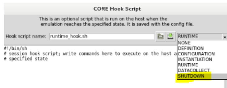
Fig. 15 CORE hook-script shutdown script
