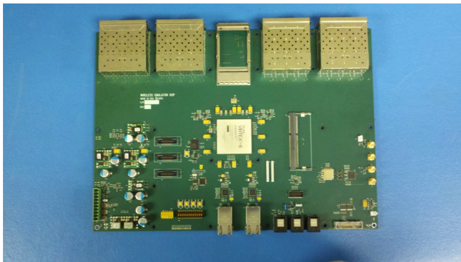
Figure 3: DSP Card
