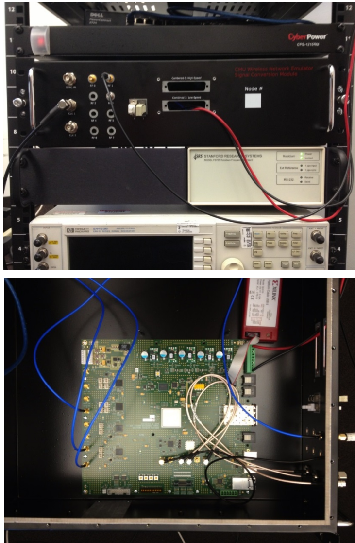
Figure 5: Front and Top view of Port Enclosures (Shows SCM)
