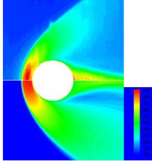
Figure 10. Comparison of experimental (top) and CFD (bottom) temperature distributions with a pulsed/DC discharge operating in plenum ( \nu=100 kHz, U_{PS}=4.5 kV). Nitrogen, P_0=370 torr. In the calculations, plenum conditions are T_0=500 K, T_{v0}=1700 K.
