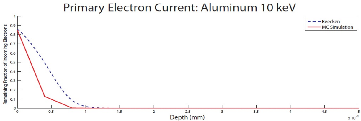
Figure 13. Comparisons of electron deposition results: BeeckenTabFred algorithm vs. Monte Carlo simulations
