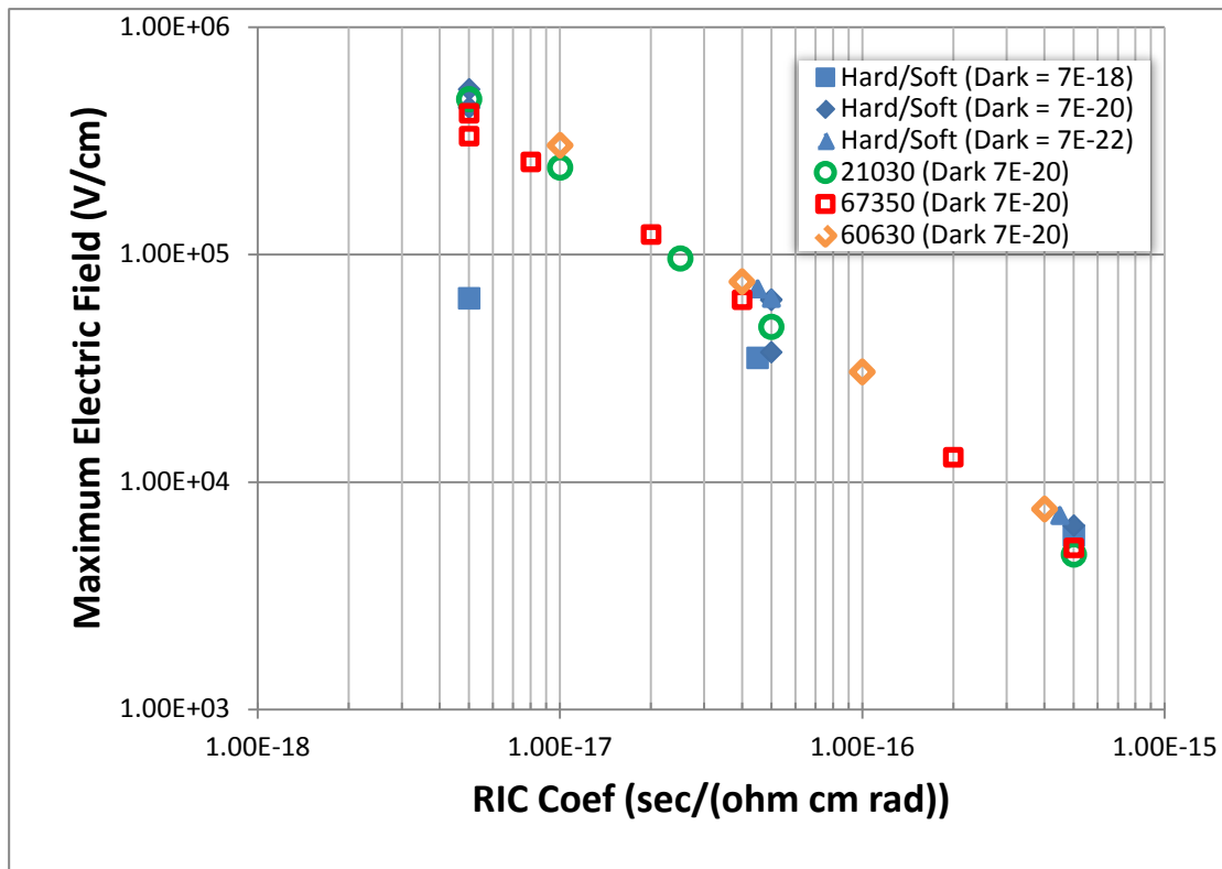
Figure 19. Summary of AF-NUMIT2 realistic simulation results
