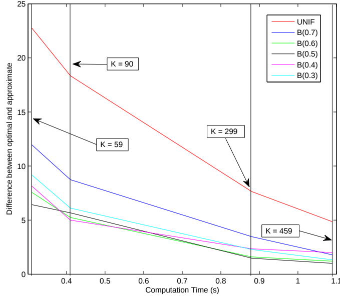
Figure 9. J^* - \tilde{J}^* by computation time
