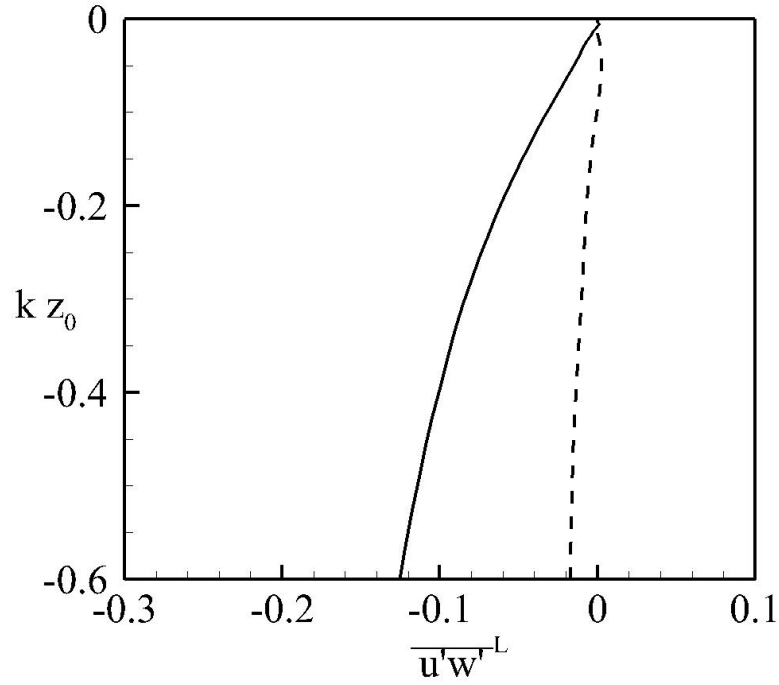
Figure 2. Vertical profiles of turbulence shear stress in Lagrangian frame for the strong wave distortion case (line) and the intermediate wave distortion case (dash).
