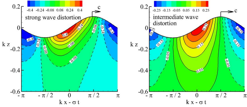
Figure 1. Contours of the normalized turbulence shear stress for the strong wave distortion case (left) and the intermediate wave distortion case (right) in the wave Eulerian frame. The arrows at the wave crest denote the wave propagation direction.
