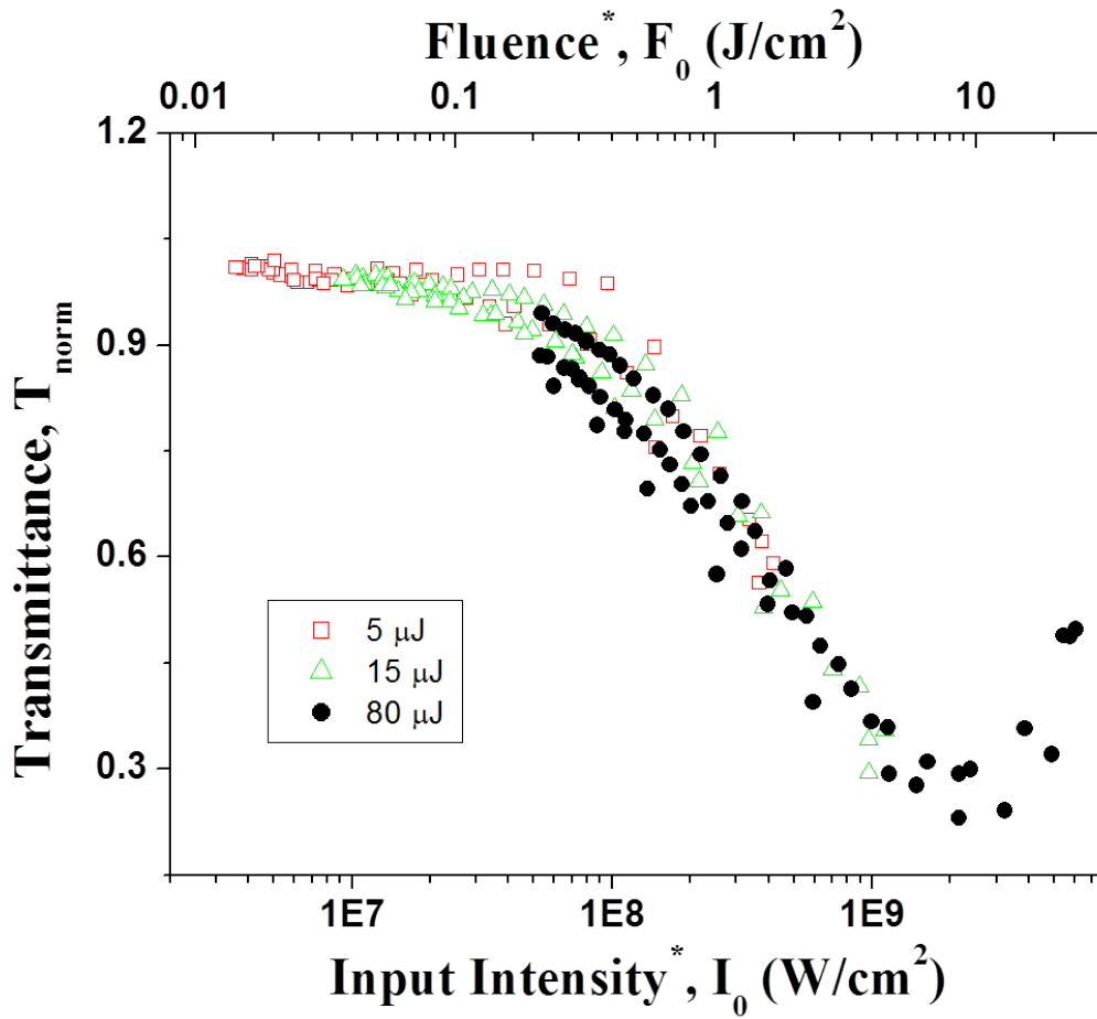
Figure 16. Evaluation of intensity (fluence) dependencies of normalized transmittance from Z-scan measurements for films of polystyrene blended with PbS nanocrystals in poly(1-butene).
