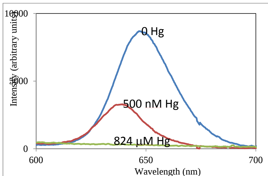
Figure 10. Fluorescence spectra of TBA probe (10 nM) without \text{Hg}^{2+} , with 500 nM \text{Hg}^{2+} , and with 824 \mu\text{M} \text{Hg}^{2+} present.
