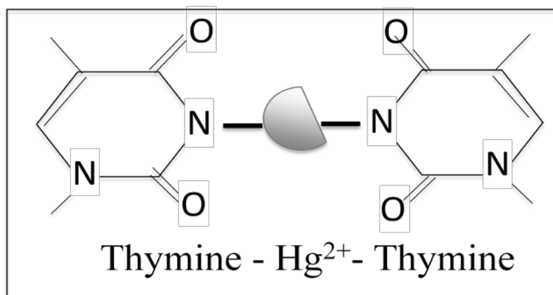
Figure 5. Mercury (II) ions interact with the nitrogen 3 atoms (N3) in the DNA base thymine.
