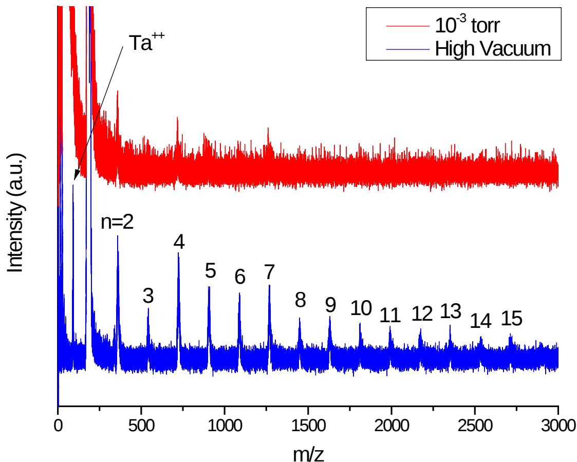
Figure 22. Tantalum cluster mass spectra from ablation by 800 nm, \sim 70 fs laser pulses at a fluence of 8 \text{ J/cm}^2 from a laser-cleaned area of chemically etched bulk Ta. Under high vacuum ( \leq 10^{-5} Torr, bottom spectrum in blue) a series of Ta clusters to at least \text{Ta}_{15} are observed within factors of 1-3 above the ablation threshold. Approaching higher pressures ( 10^{-3} Torr He, top spectrum in red) significant ion suppression and collision induced dissociation is observed, and only a few clusters are seen.
