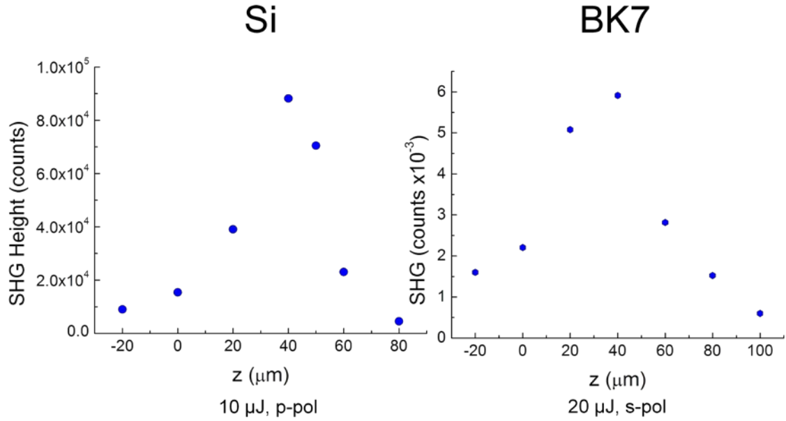
Figure 8. Double pulse SHG vs. focal distance
