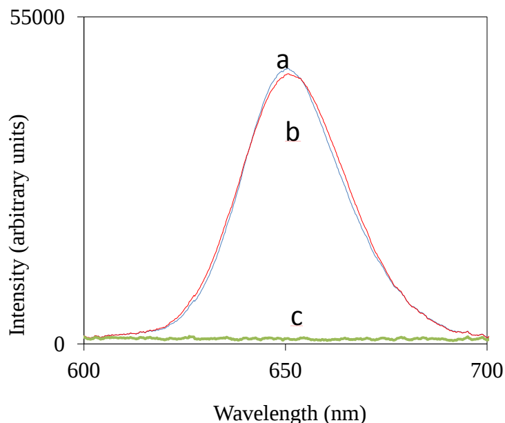
Figure 11. Fluorescence spectra of (a) QDs (10 nM), (b) QDs (10 nM) with \text{Hg}^{2+} (500 nM), and (c) QDs with \text{Hg}^{2+} (824 nM) present.
