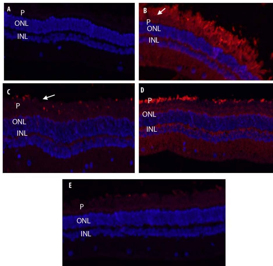
Figure 10. Autoantibody confirmation
