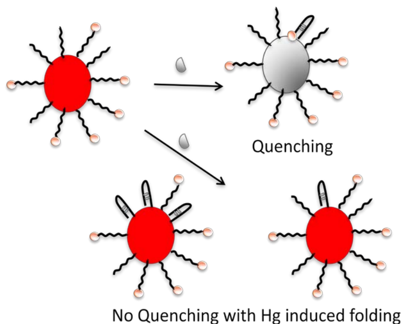
Figure 13. Actual probe configuration when using 10:1 DNA to QD ratio. Possible scenario if DNA does not have gold nanoparticle attached, which would cause a false negative.
