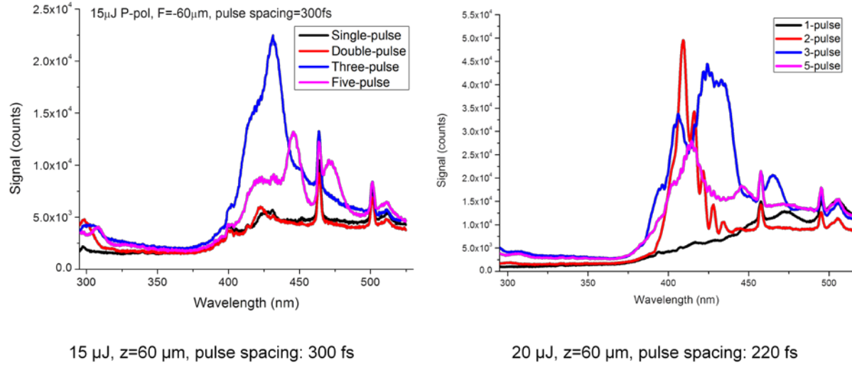
Figure 10: Plasma emission from BK7 produced by complex pulse trains
