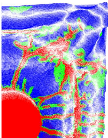
A 3 rd set of E2C cracks is generated by the first crease Symmetrical cracks form on the lower-right quarter of the plate.
