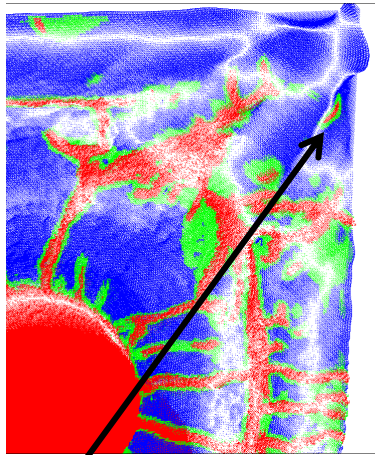
A 3 rd set of E2C cracks is generated by the first crease Symmetrical cracks form on the lower-right quarter of the plate.
