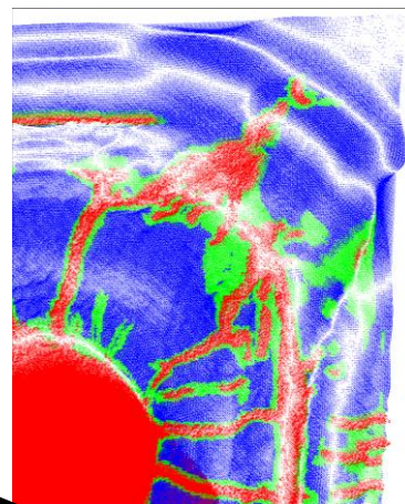
Second "crease" (due to R-wave reflection) results in localization of damage into cracks
