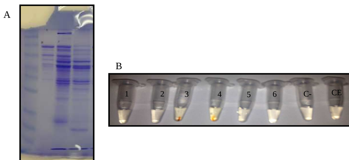
Figure 5. Selenite reduction assay for the fractions obtained from DEAE-Sepharose Fast Flow column. (A): SDS-Page of the 2 fractions with selenite reduction activity (3 and 4). MW: molecular weight marker. (B) Each tube with a number represents a fraction eluted from DEAE- Sepharose Fast Flow column. CE is the positive control (Crude extract) and C- is the negative control without fraction. Tubes with red precipitate are positive for the selenite reduction (3 and 4).
