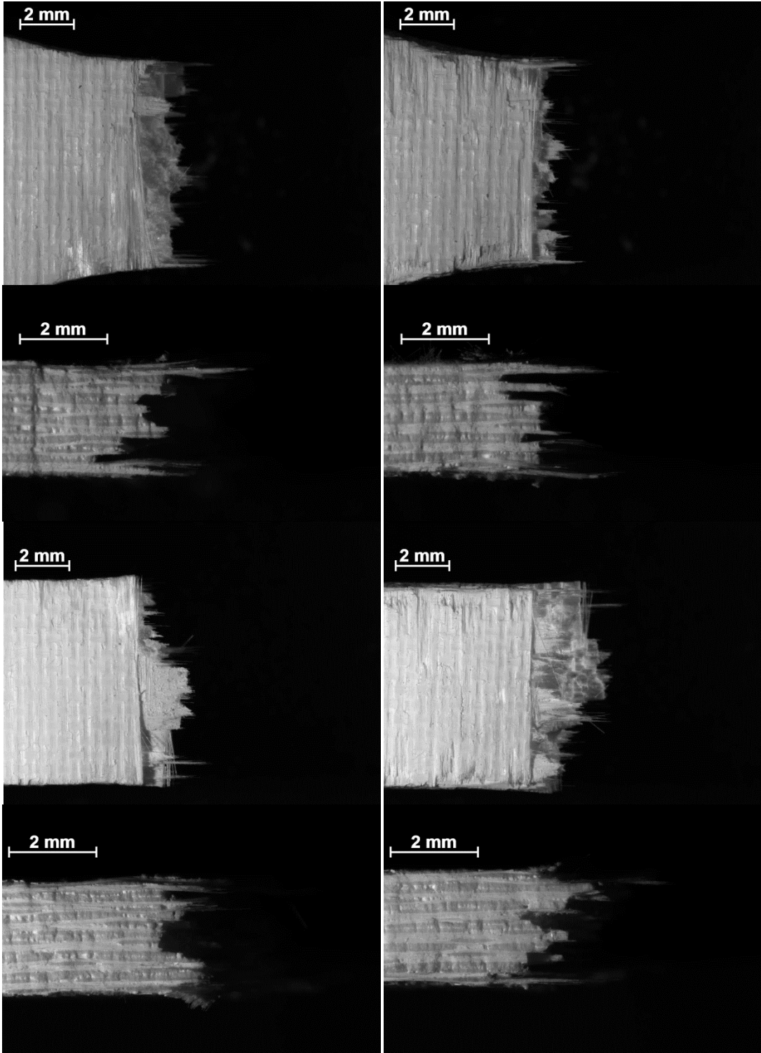
Figure E.11 - Optical micrographs of fracture surface of N720/A composite obtained in tensile tests after prior heat treatment of 100 h at 1300°C (Specimen 6)
