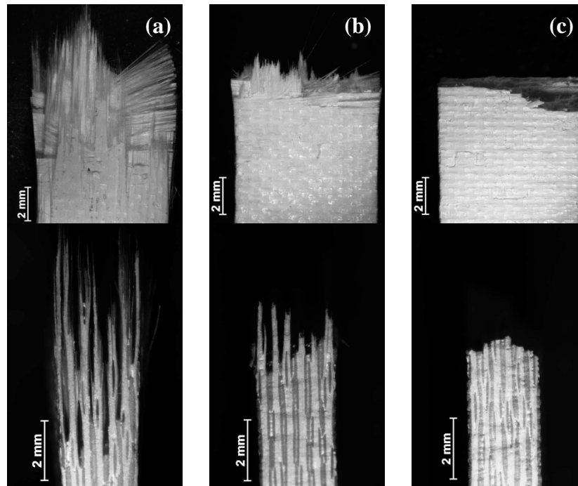
Figure 33 – Fracture surfaces of the N720/AS composite obtained in tensile tests. (a) as-received composite, (b) composite heat treated for 100 h at 1100°C, and (c) composite heat treated for 100 h at 1200°C
