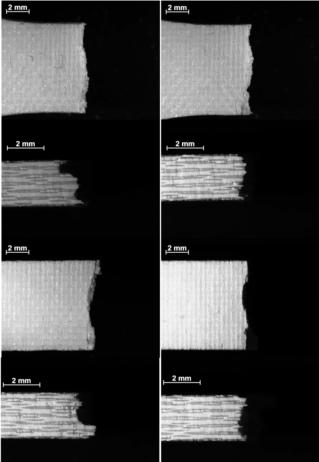
Figure D.9 - Optical micrographs of fracture surface of N720/AS composite obtained in tensile tests after prior heat treatment of 40 h at 1200°C (Specimen 5)
