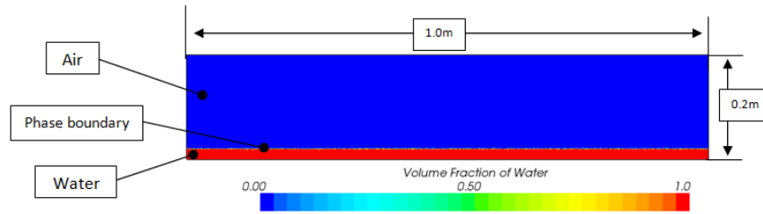
Figure 2 Phase boundary of two-phase fluid in computational domain
