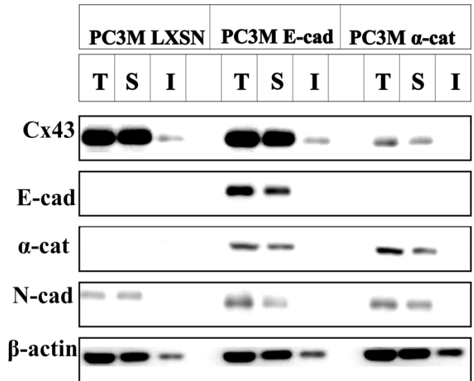
Figure 7. Expression of \alpha -catenin ( \alpha -cat) and E-cad does not alter the detergent (TX-100)-solubility of Cx43. PC3M cells were infected with the control (PC3M-LXSNS), E-cad-WT-harboring (PC3M E-cad) and \alpha -cat-harboring (PC3M \alpha -cat) recombinant retroviruses were seeded in petri dishes and confluent cells were subjected to TX100-solubility assay, followed by Western blot analysis, which biochemically measures the assembly various cell junction-associated proteins. Note that Cx43, \alpha -cat, E-cad and N-cad remain TX100-soluble even though they are detected at cell-cell contact areas (see Figure 6). TX100 = TritonX-100. T, S, and I refer to total, Tx100-soluble and TX100-insoluble fractions of cell lysates.
