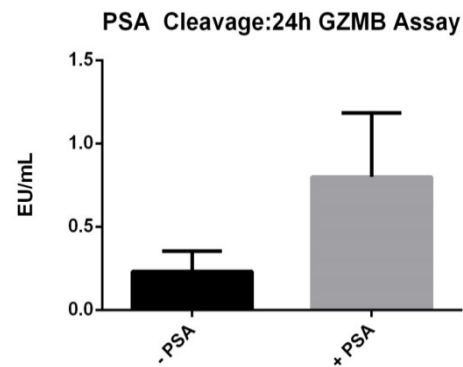
Figure 5: PSA-C248 enzymatic activity increases with PSA.
