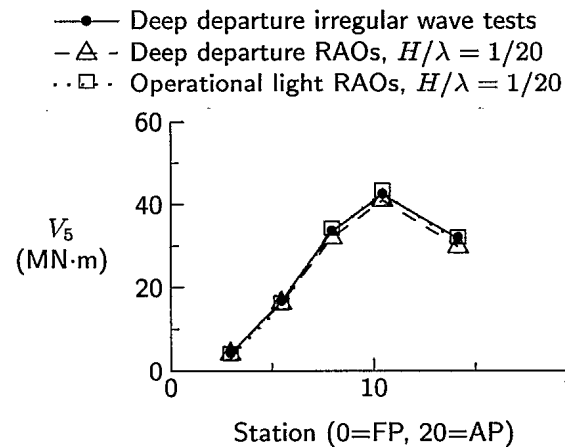
Figure 15: RMS Vertical Bending Moment Distribution in Irregular Head Seas for Deep Departure and Operational Light Conditions, H_s = 5 m, T_p = 11 s, Fn = 0.12
