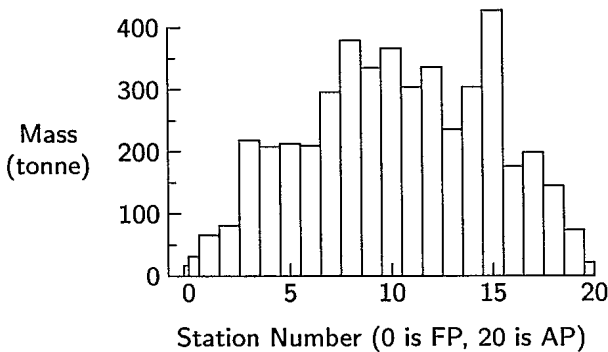
Figure 4: Sectional Mass Distribution
