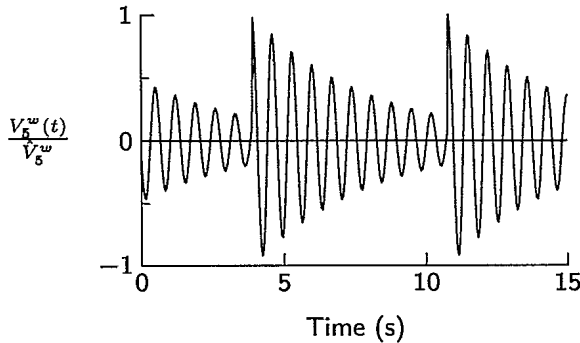
Figure 19: Time History of Idealized Whipping Response in Regular Waves
