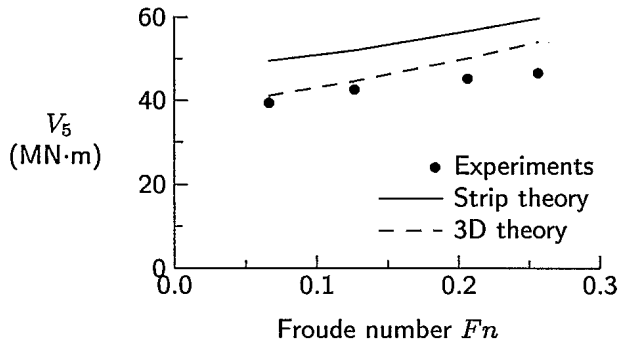
Figure 12: RMS Vertical Bending Moment at Midships Versus Froude Number in Irregular Head Seas, H_s = 5 m, T_p = 11 s
