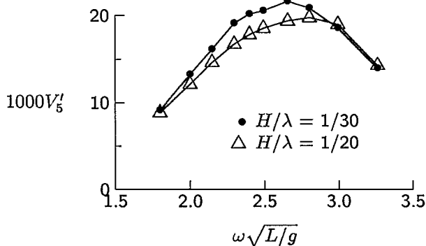
Figure 24: Wave-Induced Vertical Bending Moment at Midships, Regular Head Seas, F_n = 0.20
