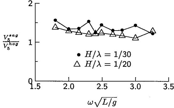
Figure 18: Wave-Induced Sag/Hog Ratio, Head Seas, Fn = 0.12
