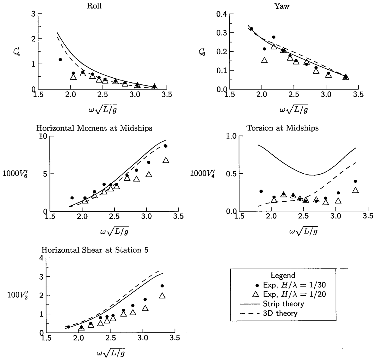
Figure 8: Lateral Plane Responses in Regular Waves, Oblique Seas, \beta_s = 135 degrees, Fn = 0.12
