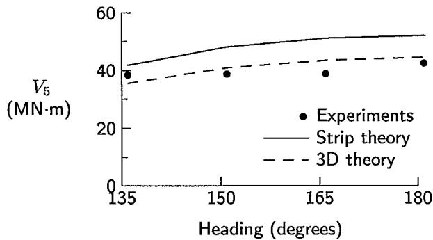
Figure 13: RMS Vertical Bending Moment at Midships Versus Heading in Irregular Seas, H_s = 5 m, T_p = 11 s, Fn = 0.12
