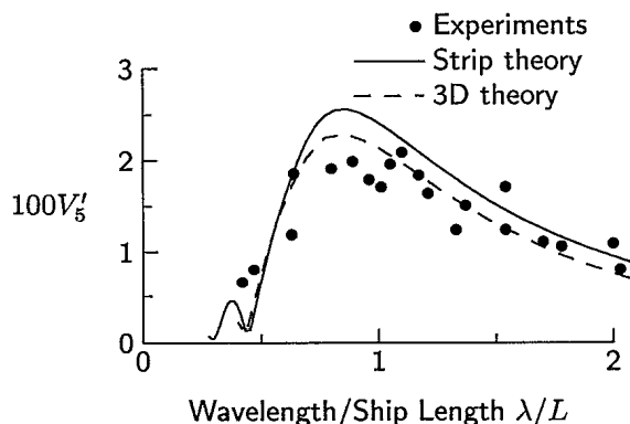
Figure 6: Vertical Bending Moment at Midships in Regular Head Seas for Warship at Fn = 0.21
