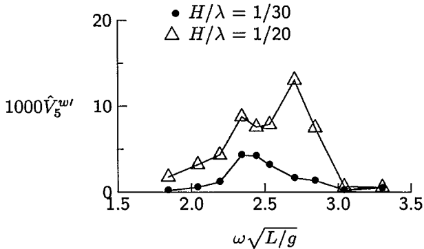
Figure 23: Maximum Whipping Moment at Midships for First Vertical Bending Mode, Regular Head Seas, F_n = 0.20
