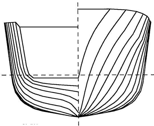
Figure 2: Body Plan for CPF Hydroelastic Model
