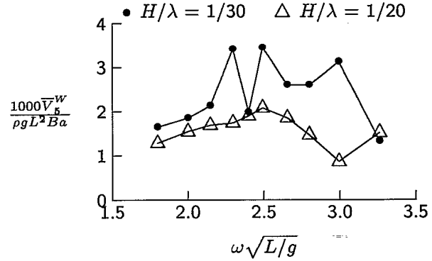
Figure 17: Midships Mean Sag Due to Waves, Head Seas, F_n = 0.12
