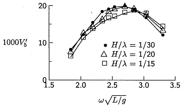
Figure 22: Wave-Induced Vertical Bending Moment at Midships, Regular Head Seas, F_n = 0.12
