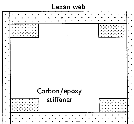
Figure 1: Cross-Section of Composite Model Backbone
