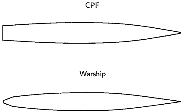
Figure 5: Waterplanes for CPF and Warship of Lloyd et al.
