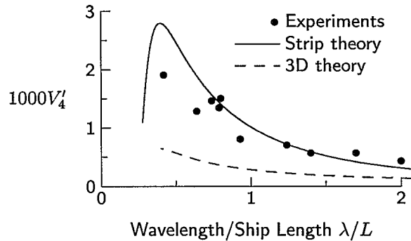
Figure 11: Midships Torsion in Regular Seas for Warship at Fn = 0.21 , \beta = 60 degrees
