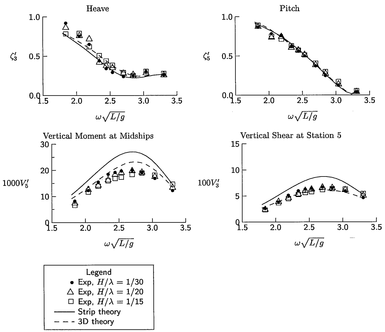
Figure 7: Vertical Plane Responses in Regular Waves, Head Seas, Fn = 0.12
