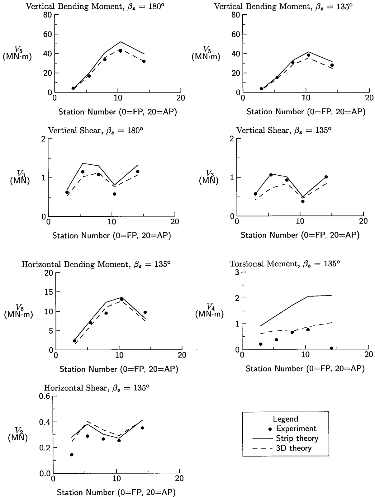
Figure 10: RMS Sea Loads in Irregular Waves, H_s = 5 m, T_p = 11 s, Fn = 0.12
