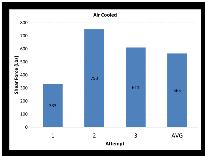
Figure 10: Maximum loading and Average for Three Trials of 10 min heat treatment cure, 1 square inch Kevlar Patch, air cool, and concrete.
