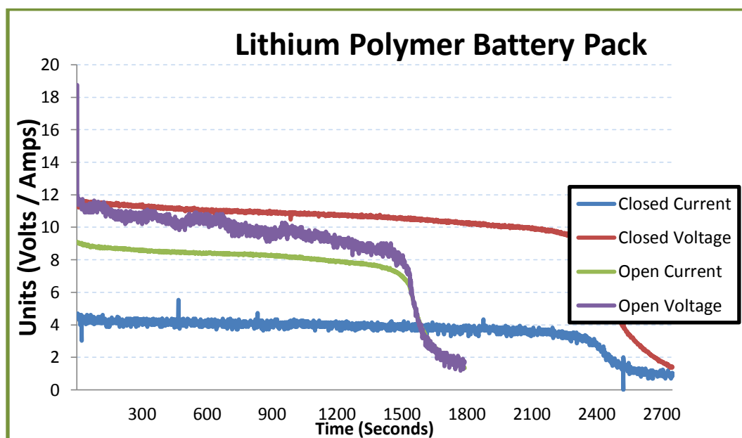
Figure 4: Li-PO Results
