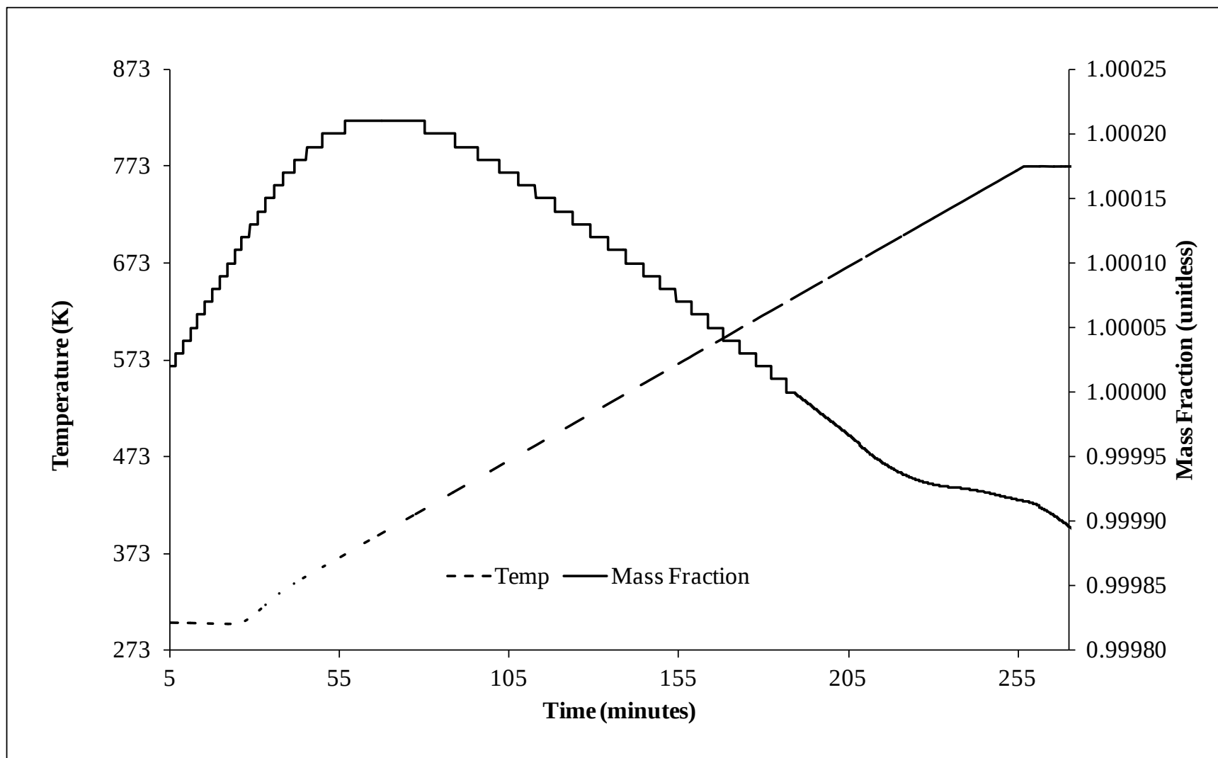
Figure 14. Copper Exposed to Deionized Water TGA Mass Loss Profile, Displays Mass Gain and Loss versus Temperature and Time
