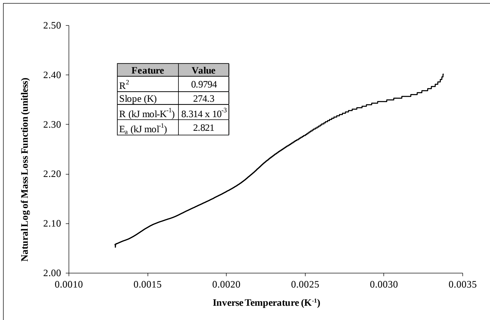
Figure 17. Copper Exposed to Malathion in Water Arrhenius Plot, Straight Line Suggests Mass Loss is First-Order
