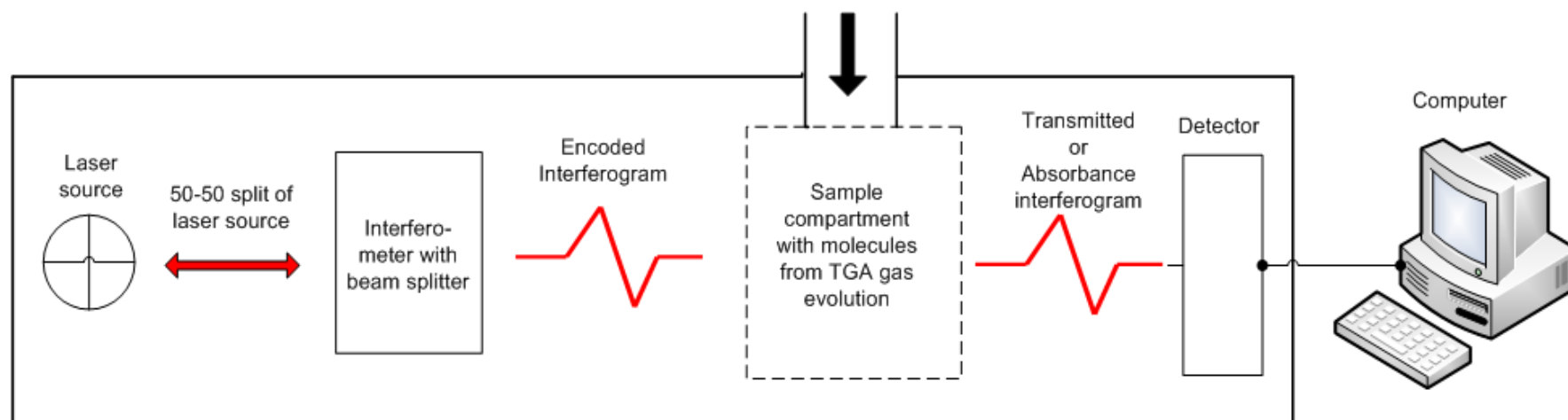
Figure 8. FT-IR System of Operations
