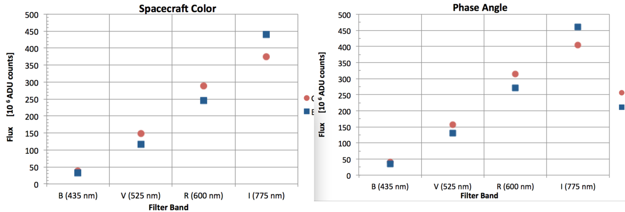
Figure 6. (Left) Intensity data for each band looking at the gold irridite and black anodized portion of the spacecraft. (Right) Intensity data in each band at two slightly different phase angles.
