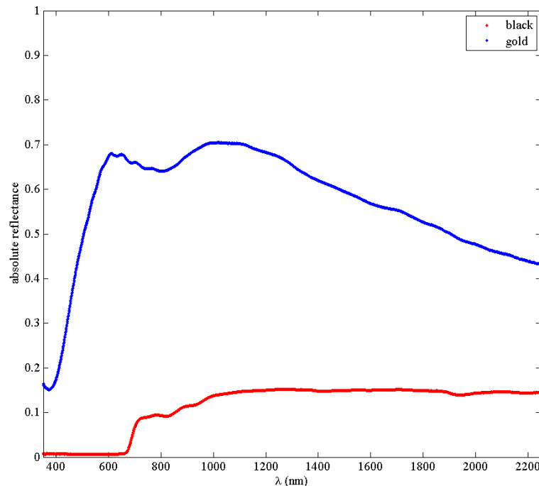
Figure 4. Mean spectral measurements for SpinSat surface, absolute reflectance versus wavelength (nm).
