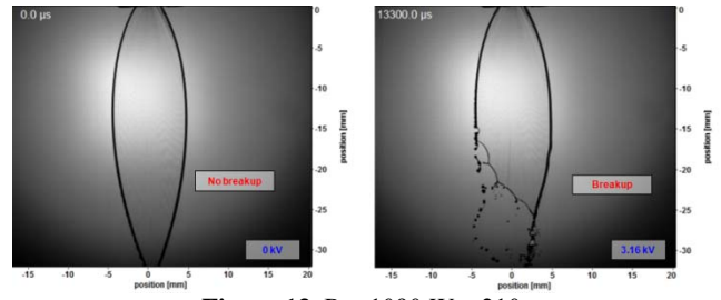
Figure 13. Re=1090, We=210
