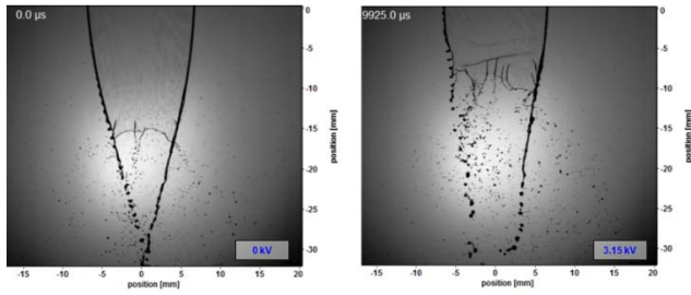
Figure 16. Re=1550 We=440
