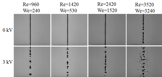
Figure 18. Array of USMA injector spray with and without electrical charge at increasing Reynolds numbers at 201 nozzle diameters below the exit plane.
