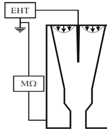
Figure 1. Spray triode [6]
