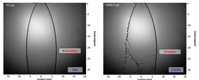
Figure 14. Re=1550, We=440
