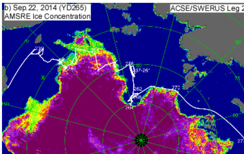
Figure 2: Track of the R/V Oden during Leg 2 of the ACSE cruise (white line) and the approximate location of the Mirai (green X) during its September deployment. Day of the year is indicated at intervals along the Oden track. The background map is the AMSRE ice concentration on Sep. 22, with purple indicating close to 100% concentration. Track positions after Sep. 24 are estimated
