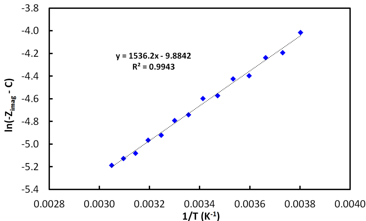
Figure 16. Linear rearrangement of Arrhenius-like equation (Equation 10) for low temperature impedance correlation of Tenergy 18650 LiCoO 2 batteries, along with linear regression trendline.
