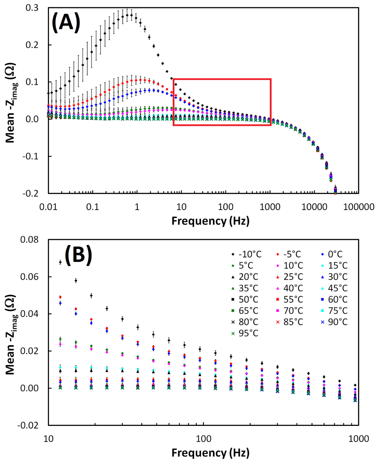
Figure 14. State of charge-averaged imaginary impedance ( -Z_{\text{imag}} ) vs. frequency for Tenergy 18650 LiCoO 2 lithium-ion batteries for temperatures between -10°C and 95°C at 5°C increments, and error bars represent standard deviations across all states of charge for each temperature. (A) shows entire range, and (B) shows zoomed in section denoted with a red box in (A) for specific range between 10-1000 Hz.
