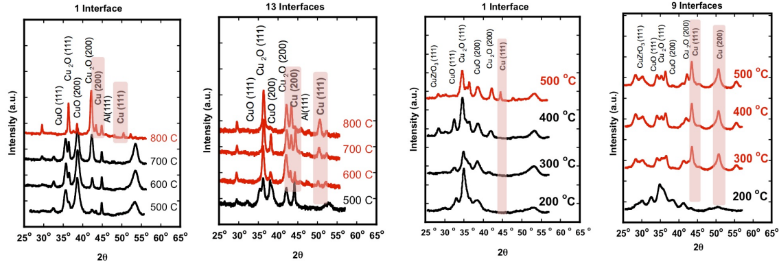
Figure 12: X-ray diffraction patterns for Al|CuO and Zr|CuO multilayers heated over a temperature ladder where the number of internal interfaces was varied while maintaining a constant sample thickness.
