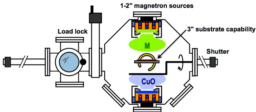
Figure 1: Schematic of NCSU dual-magnetron sputtering system optimized for naolaminate deposition
